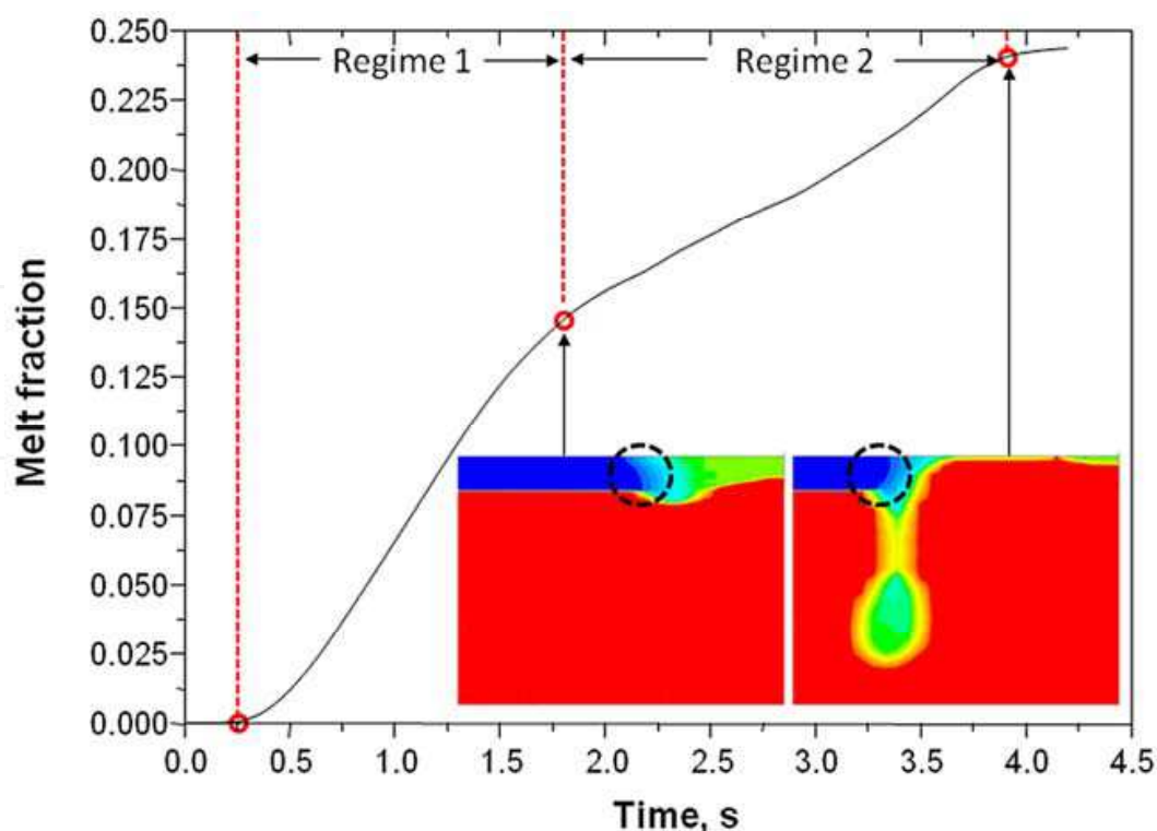
Fig. 12. Melt fraction with time, showing two regimes
