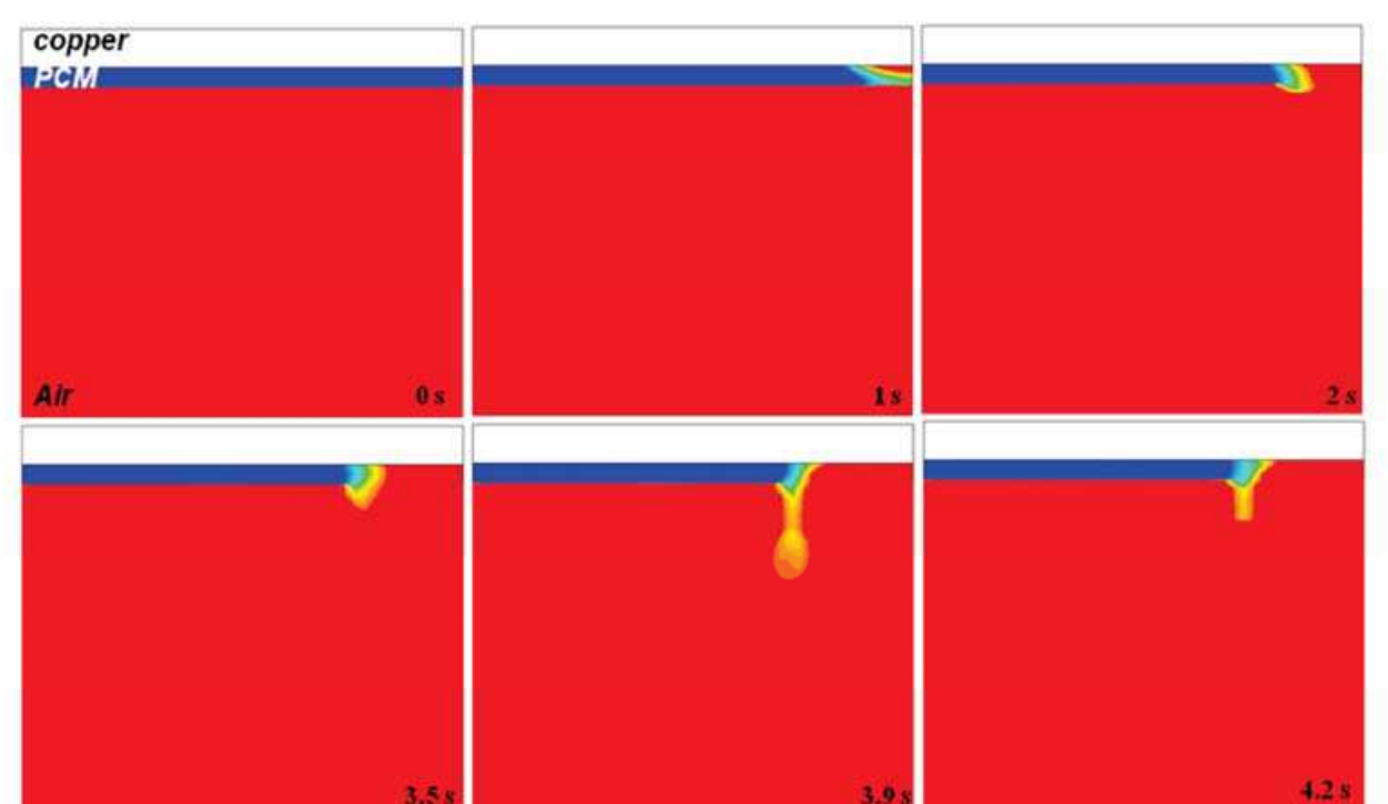
Fig. 10. Time dependence of the liquid fraction distribution
