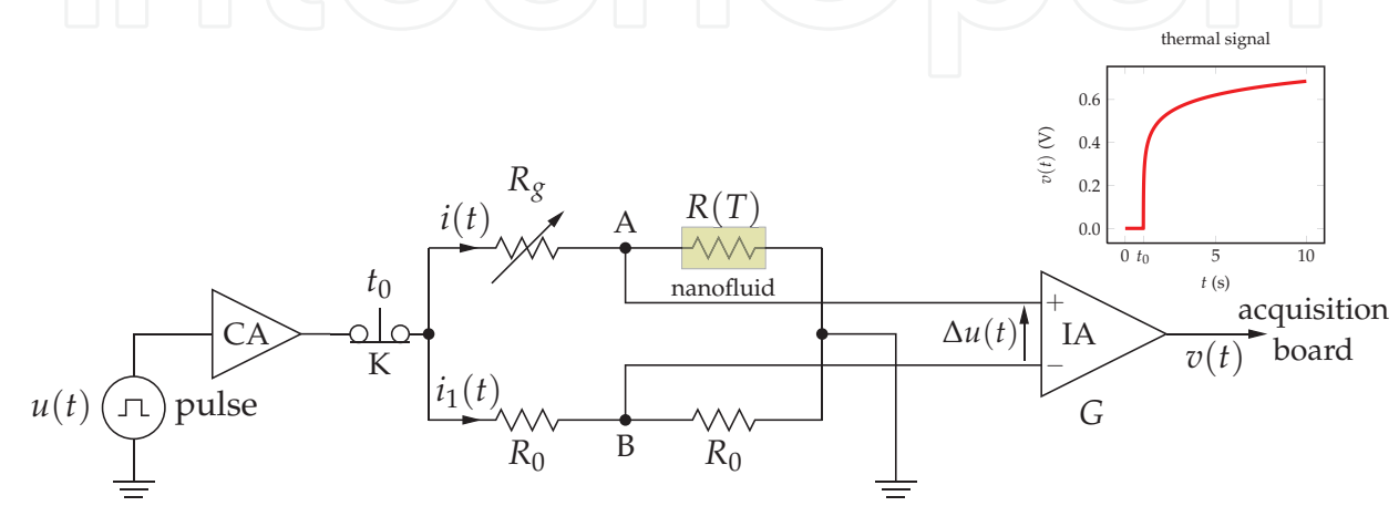
Fig. 7. THW circuit using a Wheatstone bridge.
