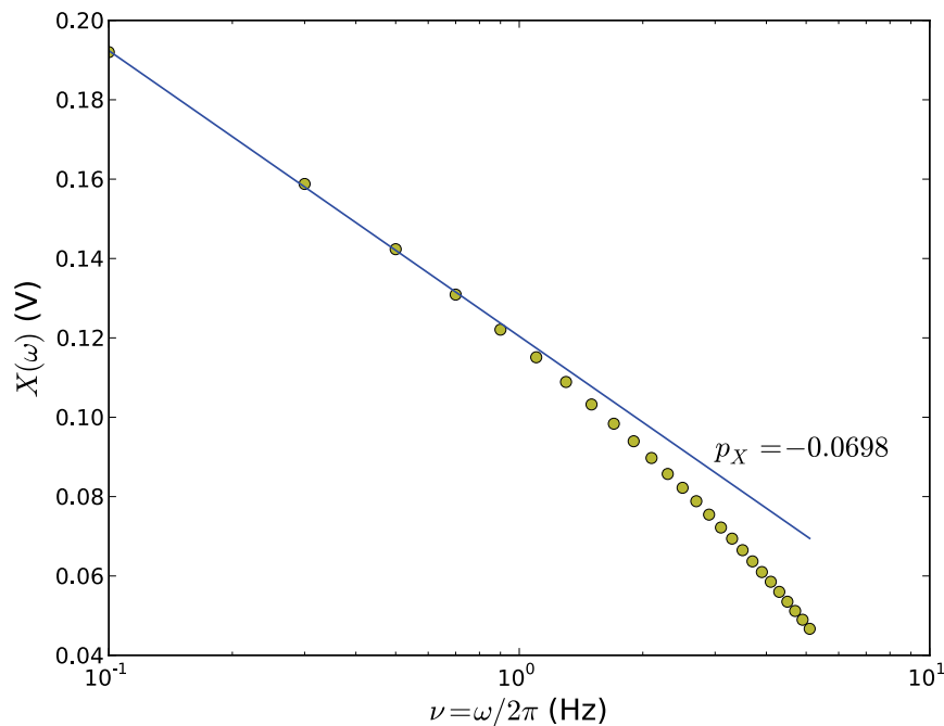
Fig. 10. Measurement of the thermal conductivity of pure glycerol at RT by the 3\omega method. Experimental values: R(T_i) = 1.430 \, \Omega , R_{\text{ref}} = 1.403 \, \Omega , G = 993 , L = 2.5 \, \text{cm} , \alpha_w = 3.92 \times 10^{-3} \, \text{K}^{-1} and \hat{I} = 148 \, \text{mA} .
