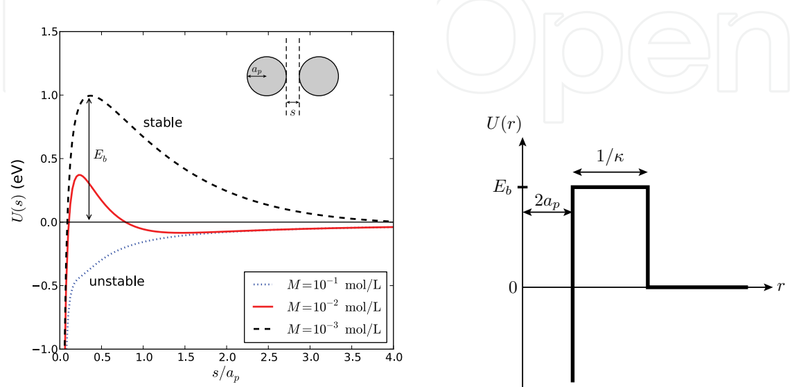
(a) DLVO interaction energy and stability tendencies of copper oxide spherical NPs suspended in water at RT and using symetric electrolytes with different molarities M and \psi_S = 0.1 V. (b) Approximate DLVO interaction potentiel used to calculate the frequency collision function K' .
