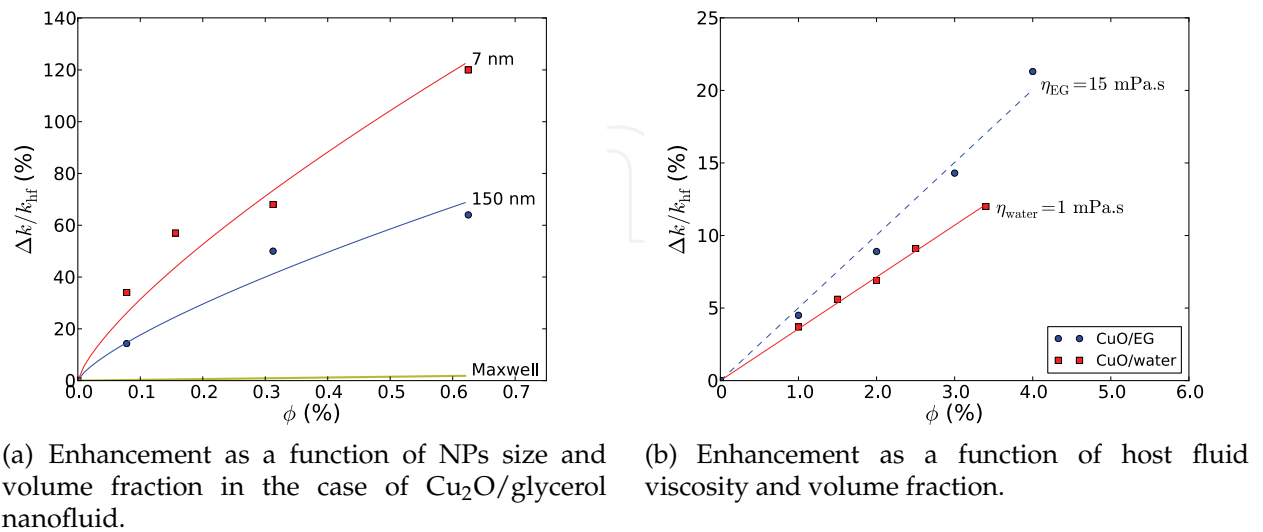
Fig. 4. Thermal conductivity enhancement of nanofluids at RT. k_{hf} is the thermal conductivity of the host fluid at RT.
