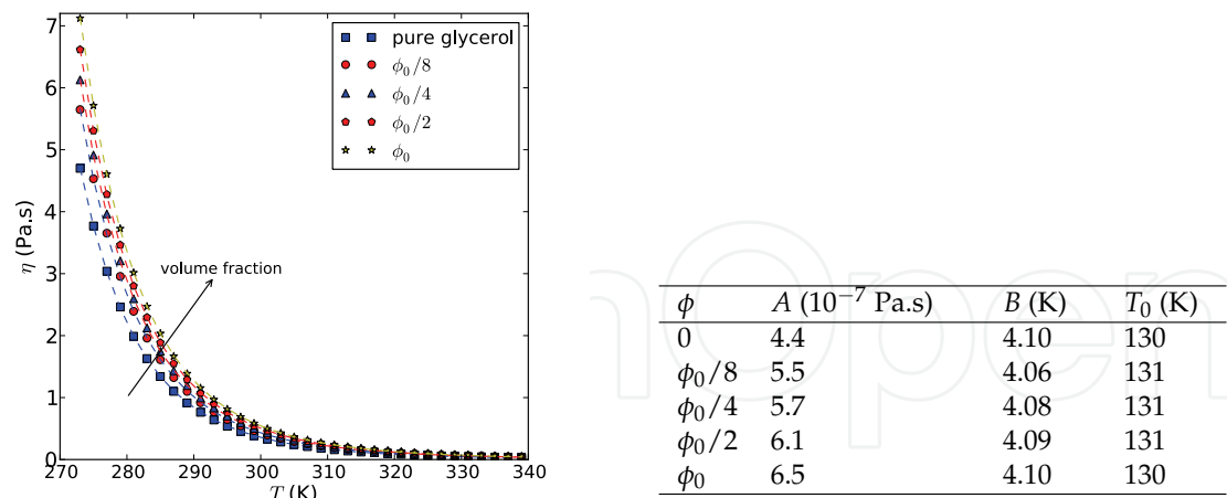
(a) Evolution of Glycerol-based nanofluids dynamic viscosity with temperature and volume fraction. \phi_0 = 0.625\% . (b) Evolution of Arrhenius law coefficients as a function of NPs volume fraction.
