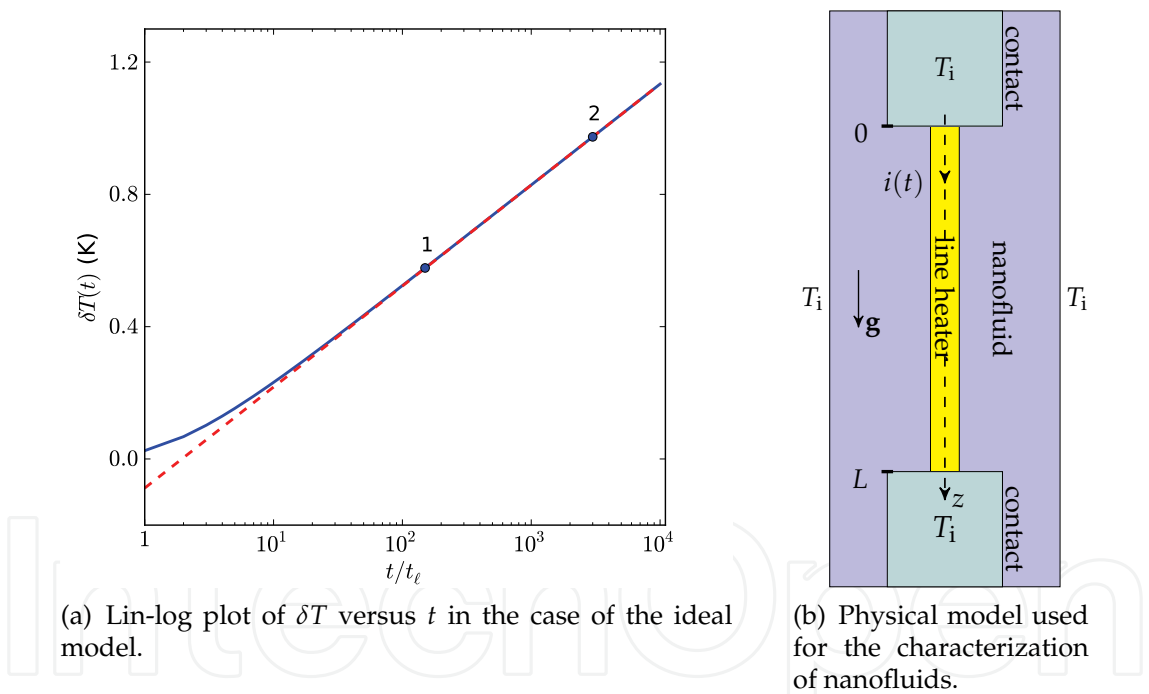
Fig. 6. Exact variation (continuous line) of the temperature rise \delta T(t) of the wire in the case of pure water with \dot{q} = 1\text{W/m} , a = 25\text{ }\mu\text{m} and using the THW technique. The amplitude of \delta T satisfies to the linear approximation.
