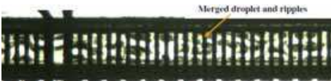
Fig. 27. A drop-wise slug flow pattern in a hydrophobic microchannel (Choi & Kim, 2008)
