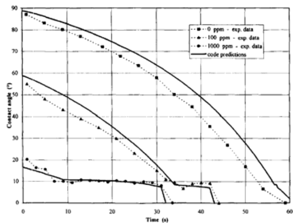
Fig. 11. Evolution of contact angle during evaporation of droplets of pure water, 100 ppm and 1000 ppm surfactant solutions on a stainless steel surface at 80 °C, (Chandra et al., 1996)
