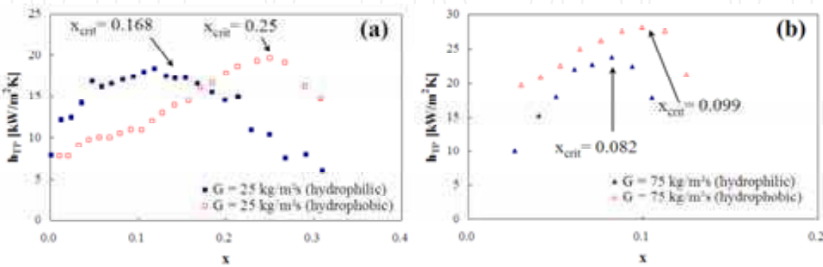
Fig. 29. A local heat transfer coefficient in rectangular microchannels for different wettabilities and mass fluxes: (a) 25 kg/m²s, (b) 75 kg/m²s (Choi et al, 2010)
