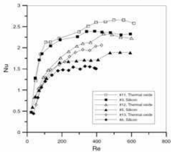
Fig. 6. Effect of surface wettability on Nusselt number: #11(L/D h ~307), #3(L/D h ~310), #12(L/D h ~368), #5(L/D h ~370), #13(L/D h ~451), #6(L/D h ~451) (Wu & Cheng, 2003)
