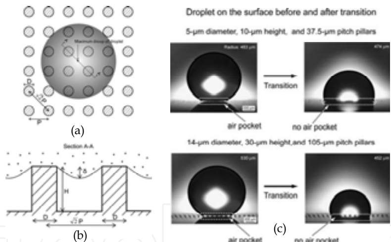
Fig. 12. A small water droplet suspended on a super-hydrophobic surface consisting of a regular array of circular pillars. (a) Plan view. (b) Side view in section A-A, (c) Visualization results for transition (Jung & Bhushan, 2007)
