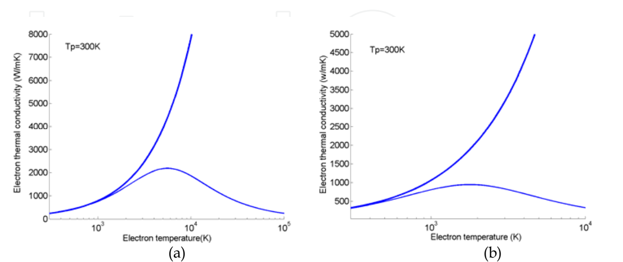
Fig. 1. The electron thermal conductivity as a function of electron temperature for the targets of Au (a) and Al (b), the thick line stands for k_{e2} , the thin line stands for k_{e1}
