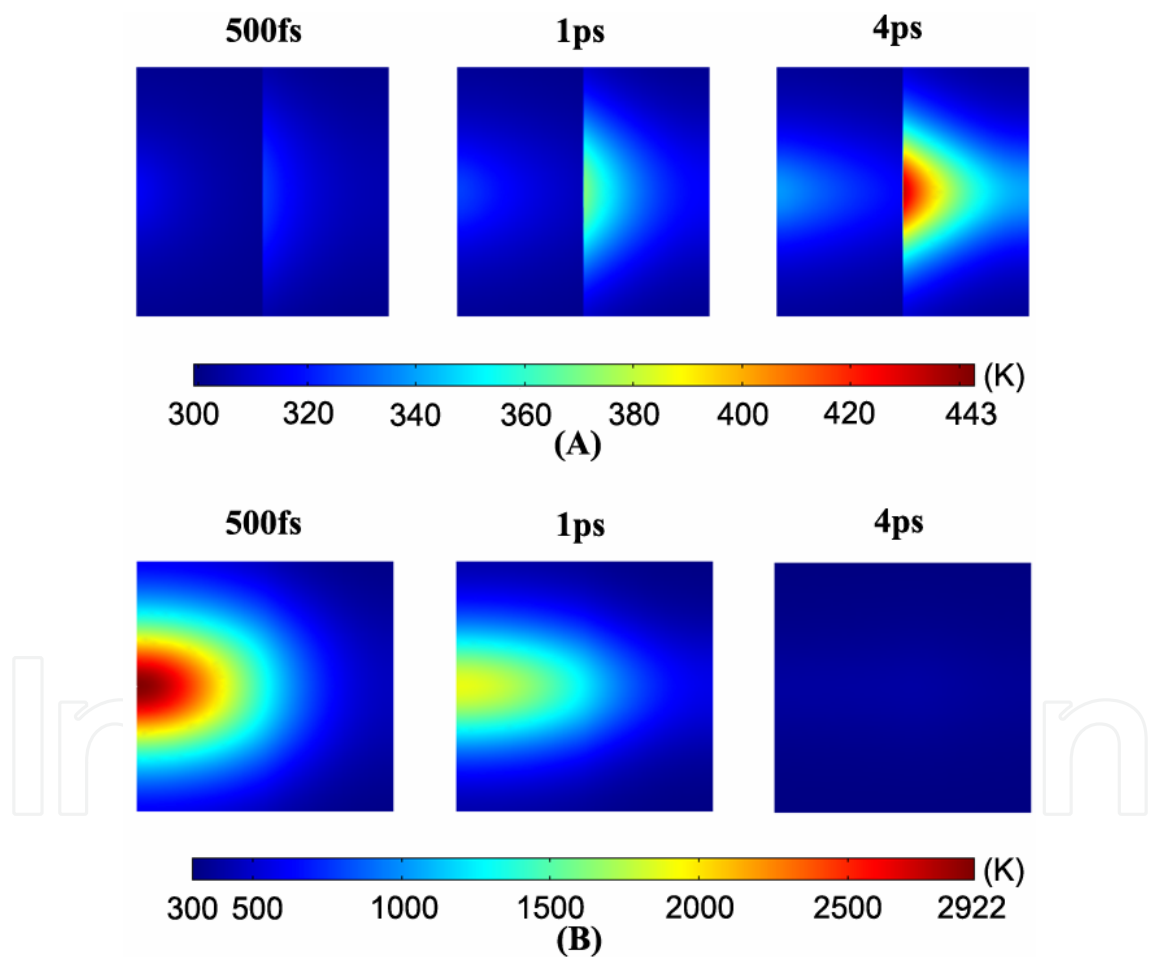
Fig. 4. The temporal evolution of electron and phonon temperature fields in two layer Au/ Al film assembly. (A) Phonon temperature fields at 500fs, 1ps and 4ps; (B) Electron temperature fields at 500fs, 1ps and 4ps
