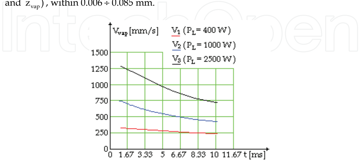
Fig. 5. The vaporization speed variation vs. processing time
