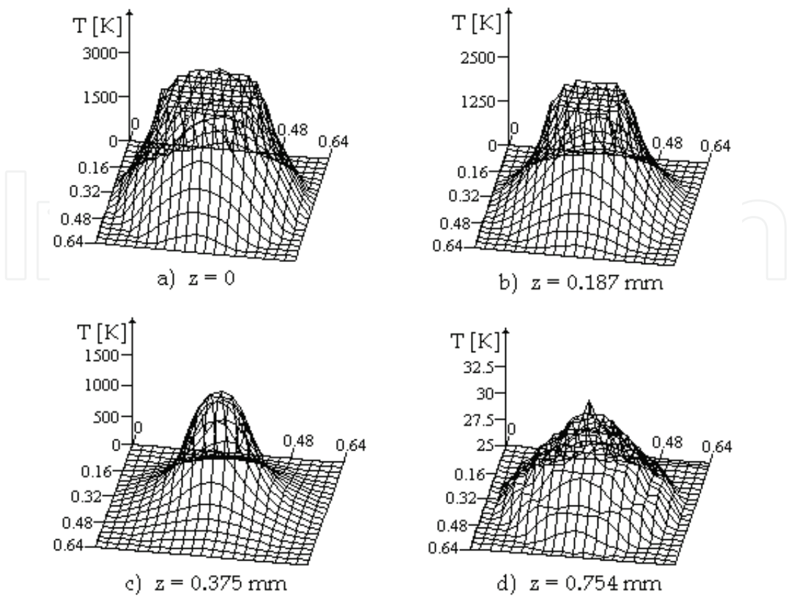
Fig. 4. Temperature distribution, P_L = 400\text{W} , t = 1\text{ms}
