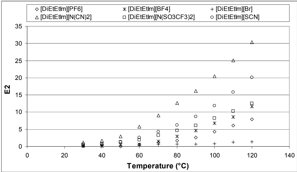
Fig. 5. Dielectric loss factor of ILs containing common [DiEtEtIm] cation and different anions
