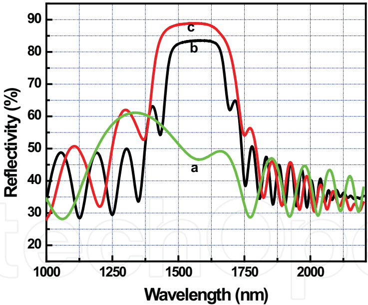
Fig. 18. Reflection spectra versus period numbers of stacks: curves a, b and c from multilayer filters with periods of 6, 18 and 12, respectively.
