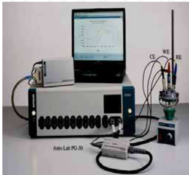
Fig. 1. Electrochemical etching setup for fabricating PS layers
