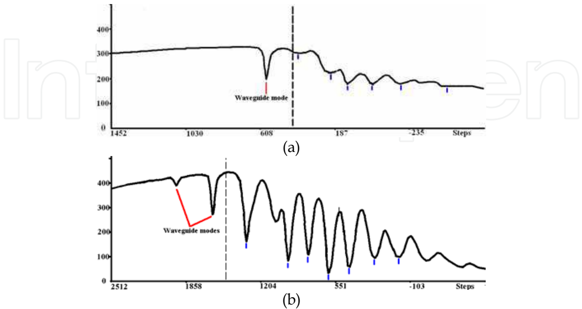
Fig. 7. Waveguide properties of the SRSO core/cladding layers. (a) Single-mode in the sample with core/cladding thickness of 1.90/6.24 \mu\text{m} and indices of 1.6088/1.5402 (b) Multi-mode in the sample with core/cladding thickness of 5.54/3.35 \mu\text{m} and indices of 1.4512/1.4275.
