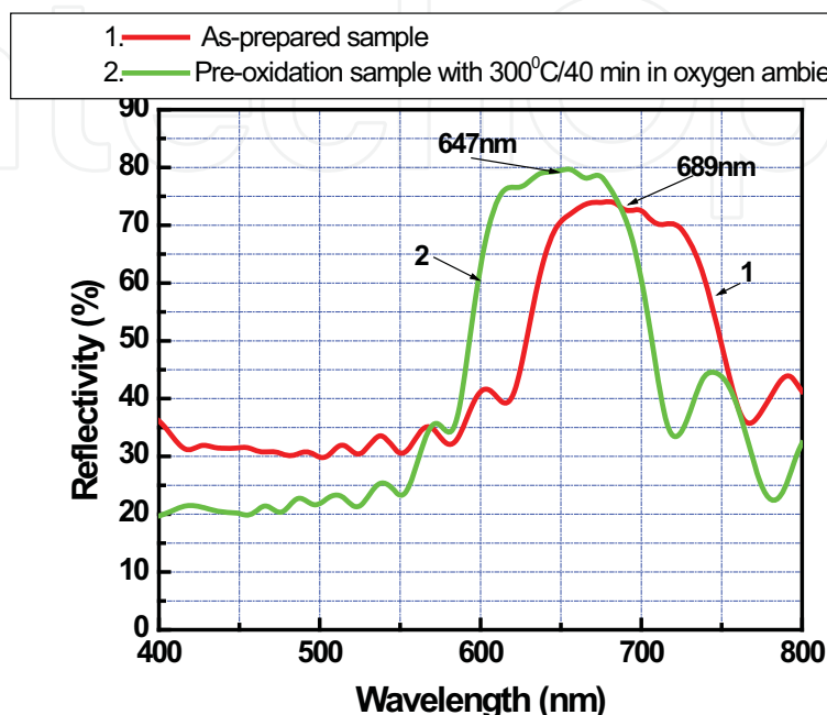
Fig. 20. Filter wavelength of as-prepared (1) and pre-oxidation (2) PS samples at 300°C in oxygen ambient. The blue-shift of filter wavelength of 42 nm was obtained.
