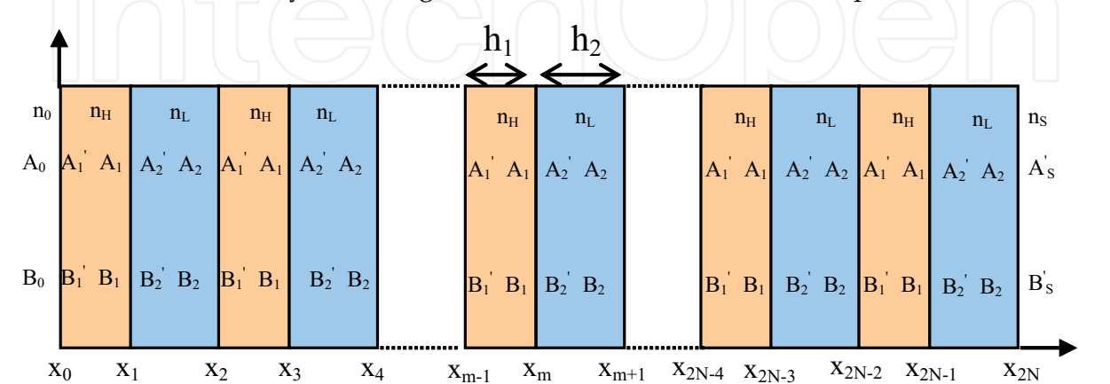
Fig. 11. Diagram of multi-layer interference filters.
