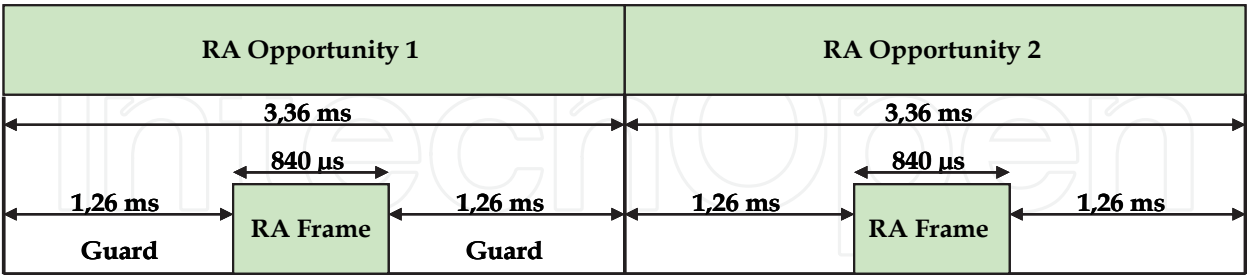
Fig. 8. Random access opportunities.
