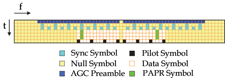
Fig. 9. Structure of random access frame.
