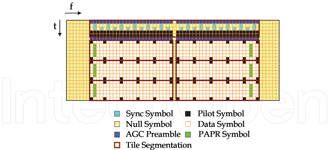
Fig. 7. Structure of one DC segment.
