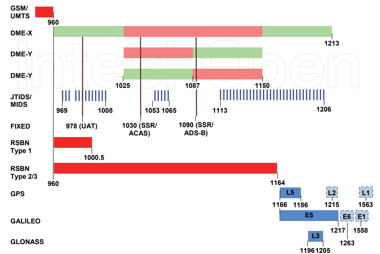
Fig. 1. Current L-band usage (SESAR JU, 2011).
