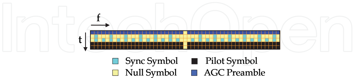
Fig. 6. Structure of one synchronization tile.
