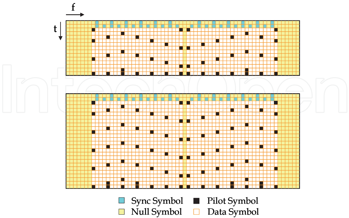
Fig. 4. Structure of BC1 and BC3 sub-frames (above) and BC2 sub-frame (below).
