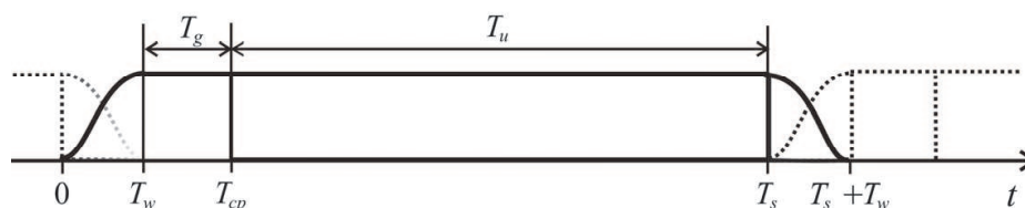
Fig. 13. Tx windowing principle.
