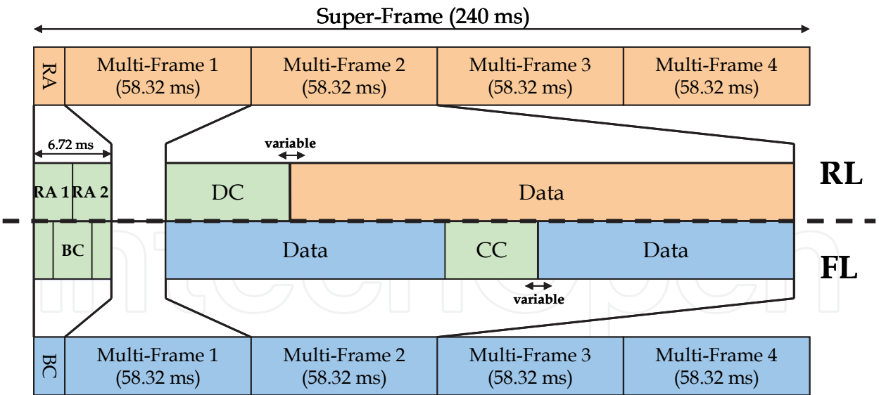
Fig. 11. Super-Frame Structure.
