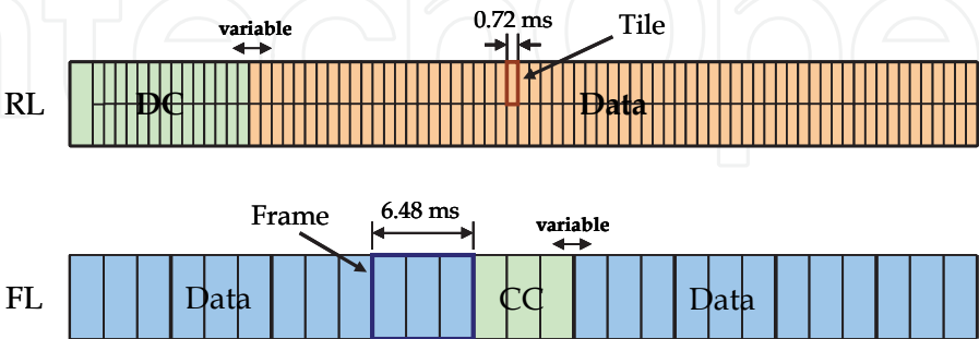
Fig. 10. Multi-Frame structures.
