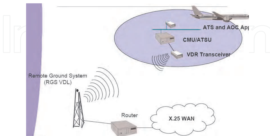
Fig. 8. VDL architecture.
