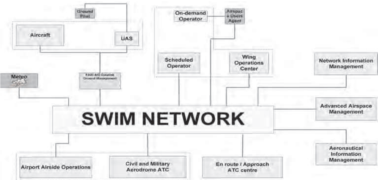
Fig. 3. SESAR SWIM architecture.
