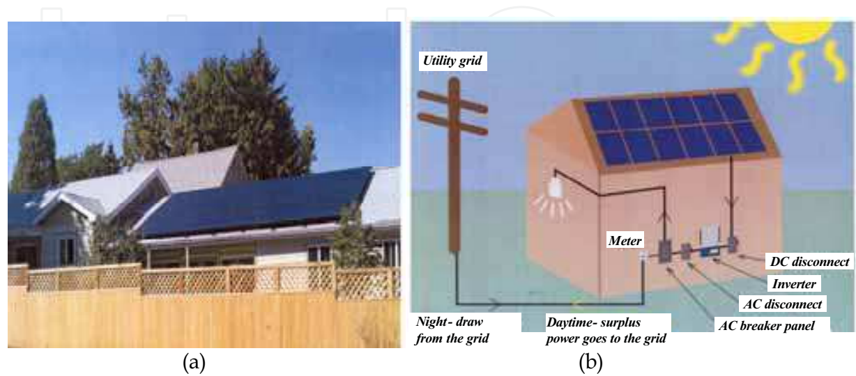
Figs. 7a,b. (a) Residence with solar panels in Boulder, CO, 2007; (b) Net metering (Courtesy of Namasté Solar, 4571 North Broadway, Boulder, CO 80304), 2007
