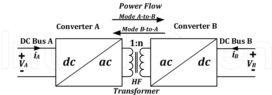
Fig. 5. Basic structure of an IBDC
