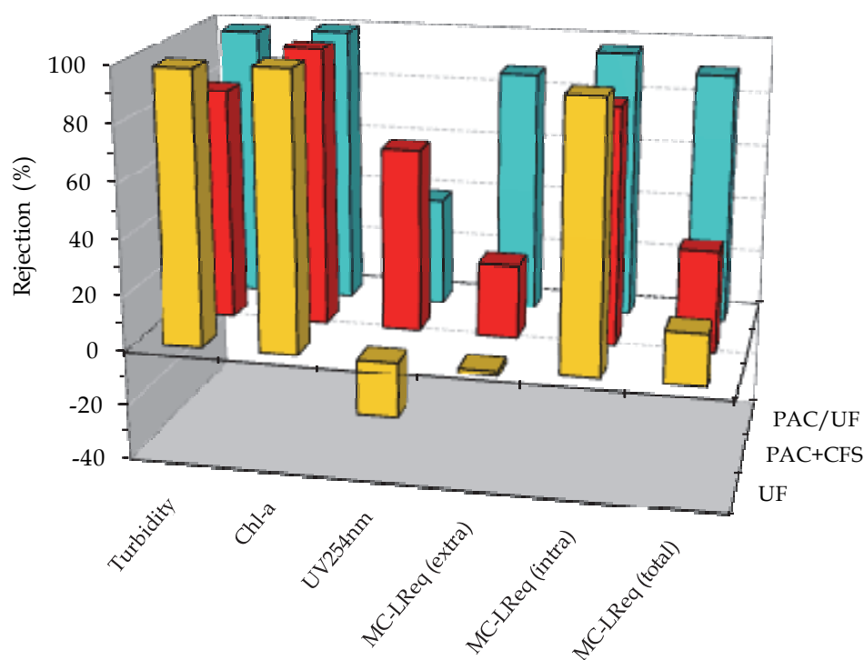
Fig. 10. UF, PAC+C/F/S and PAC/UF performances with ozonated water supplemented with M. aeruginosa culture and dissolved microcystins ( 7.2\text{--}8.5\text{ }\mu\text{g/L} MC-LReq, 4-5 extra/intracellular; 10\text{ mg/L} PAC).
