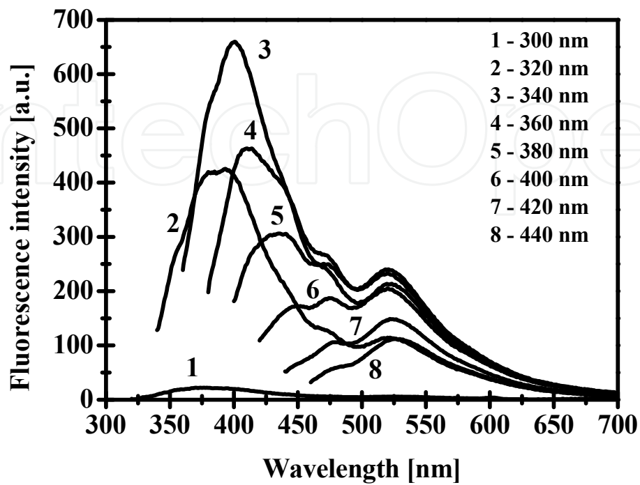
Fig. 13. Fluorescence emission spectra of all- trans \beta -carotene; c = 5 \text{ } \mu\text{M} in (IL1), \text{C}_8\text{H}_{17}\text{OCH}_2\text{-C}_1\text{Im}][\text{BF}_4] ; 10 mm cuvette; as a function of excitation wavelength.
