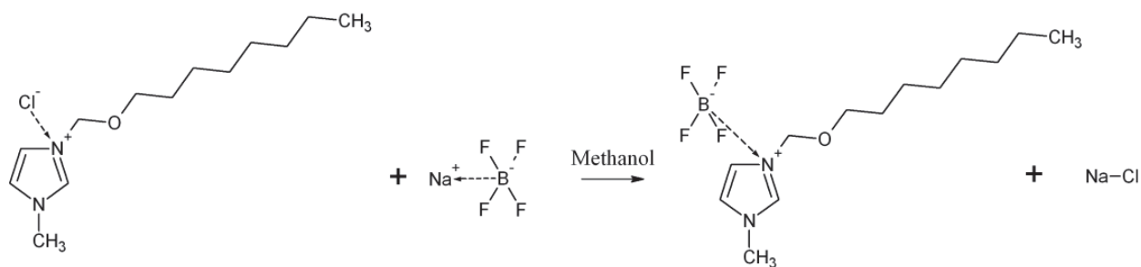
Fig. 2. Preparation of 1-methyl-3-octyloxymethylimidazolium tetrafluoroborate (IL1).
