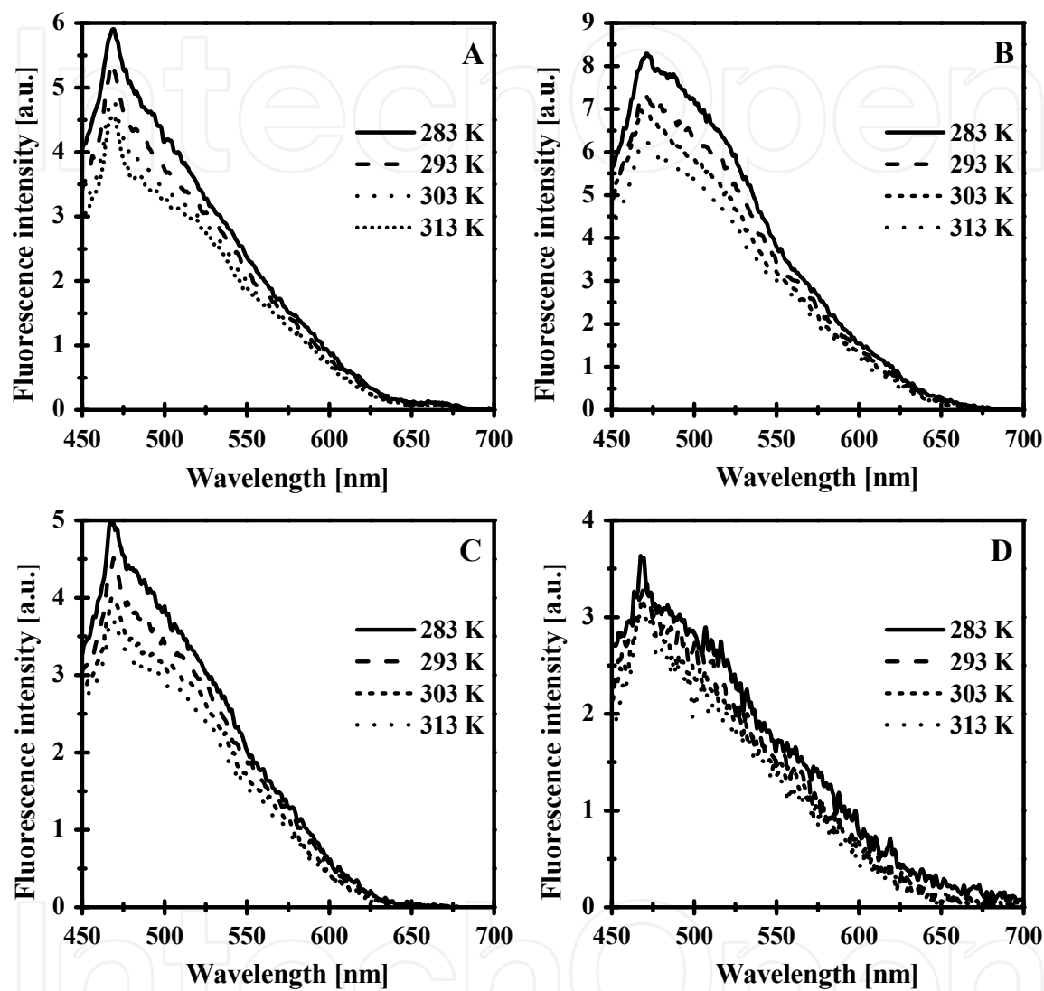
Fig. 11. Fluorescence emission spectra of: (A)- (IL1) [C 8 H 17 OCH 2 -C 1 Im][BF 4 ]; (B)- (IL2) [C 6 H 13 OCH 2 -C 1 Im][(CF 3 SO 2 ) 2 N]; (C)- (IL3) [C 8 H 17 OCH 2 -C 1 Im][(CF 3 SO 2 ) 2 N]; (D)- (IL4) [C 8 -C 1 Im][BF 4 ] (μ-cuvette) as a function of temperature.
