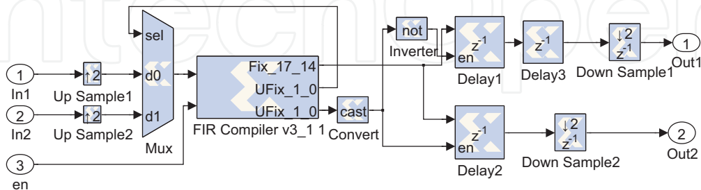
Fig. 3. Optimized blocks for applying the Doppler Spectrum.
