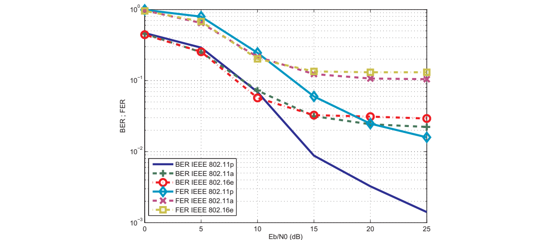
Fig. 13. Performance comparison when transmitting over VTV-Expr. Oncoming .
