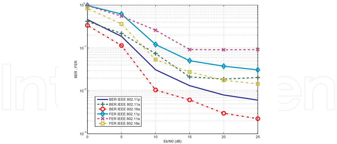
Fig. 12. Performance comparison when transmitting over RTV-Suburban Street .
