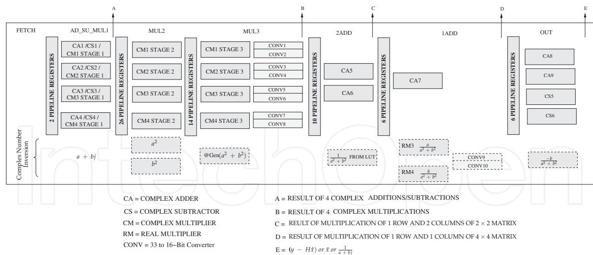
Fig. 6. CAU and pipeline stages
