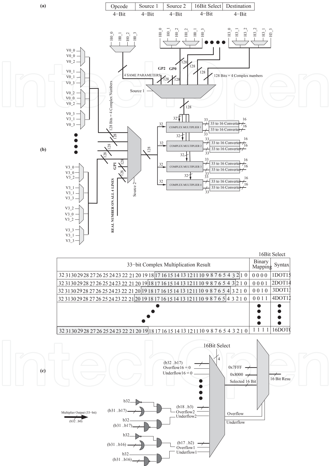
Fig. 8. Complex multiplication datapath: (a) 20-bit Multiply Instruction, (b) Possible inputs to complex multipliers, (c) 33 to 16-bit converter
