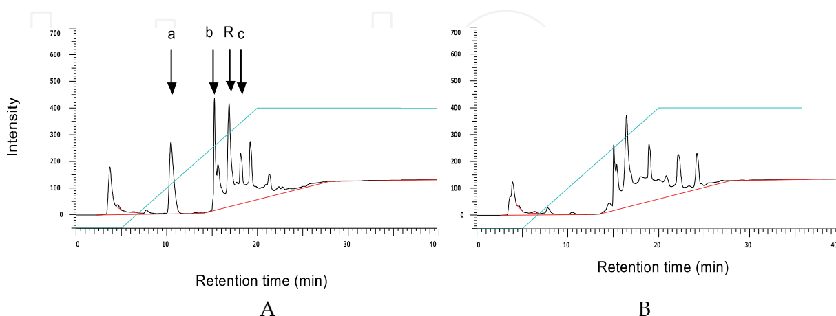
Fig. 13. Peptide uptake from degraded soybean meal products solution by the root system of Brassica rapa .
