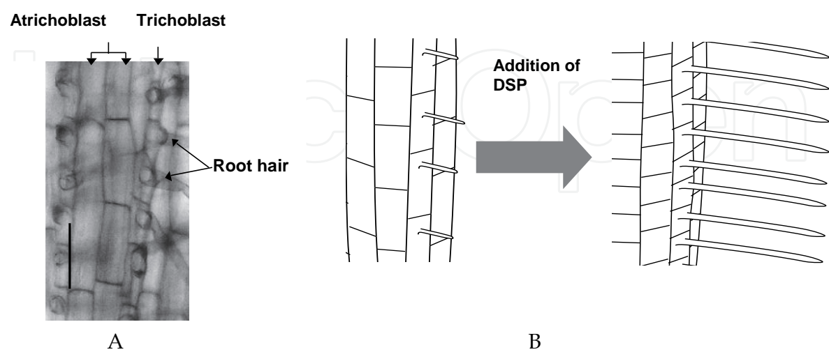
Fig. 7. Microscopic examination of root hairs grown in the presence of 30 µg/ml of degraded soybean meal products (DSP) (A) and a schematic model of the effect of DSP on trichoblast and atrichoblast (B).
