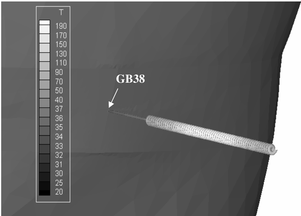
Fig. 15. The predicted skin surface temperature contours for the warm needle applied at the location near the acupoint GB38
