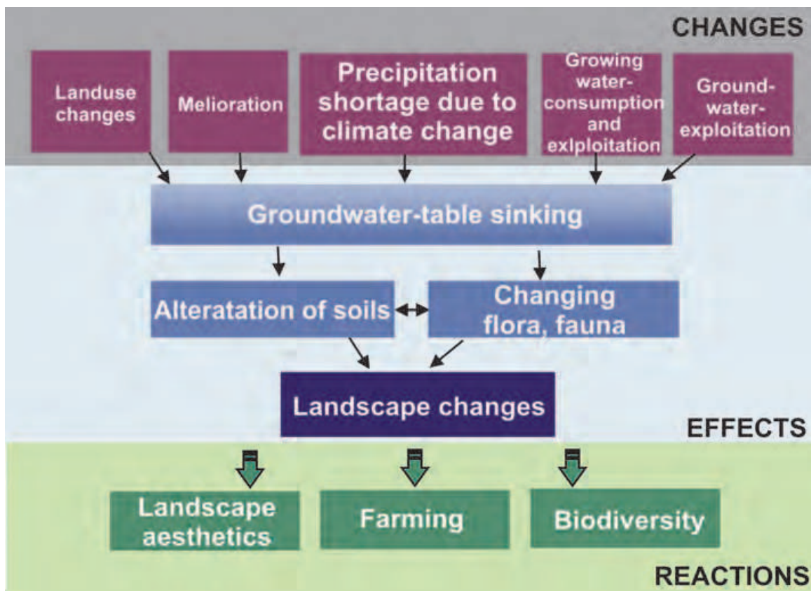
Fig. 22. The revealed relationship-system of aridification in the Danube-Tisza Interfluvium (Great Hungarian Plain) (Ladányi 2010).
