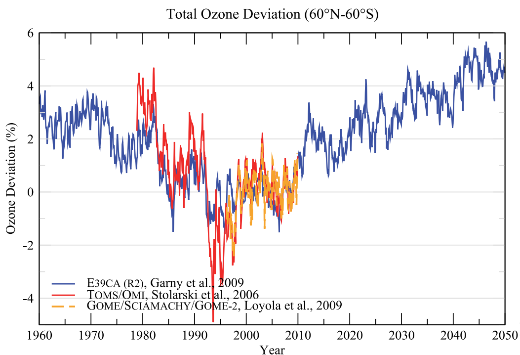
Fig. 10. Average deviations of the total ozone column (in %) for the region between 60°N and 60°S. The mean annual cycle for the period 1995-2009 was subtracted in each case. The orange and red curves represent data obtained from satellite instruments (TOMS, GOME, SCIAMACHY and GOME-2). The blue curve shows results from a numerical simulation (R2) using a chemistry-climate model (E39CA).
