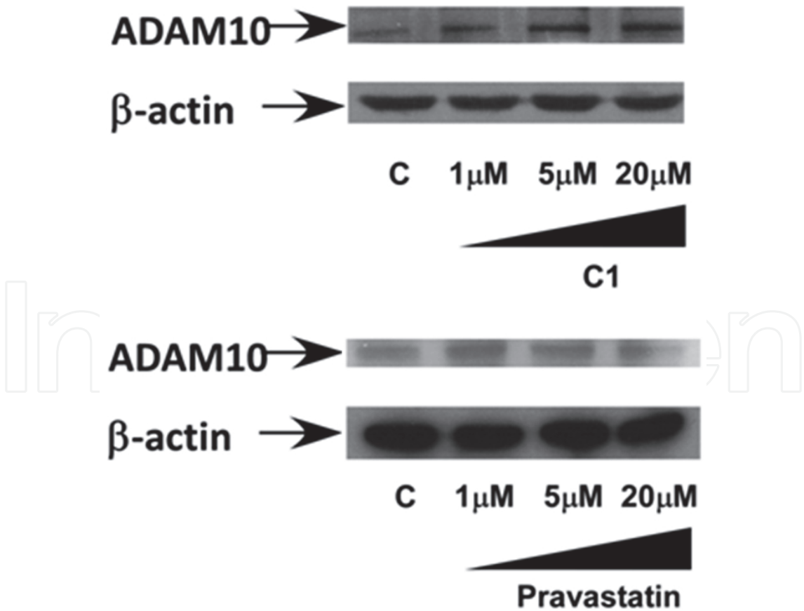
Fig. 12. Effect of escalating dose of C1 (Table 1) and pravastatin on α-secretase (ADAM10) levels in HEK293 cells. Immunoblotting performed as per Mankidy et al., 2010.
