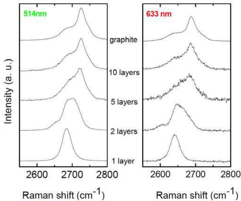
Fig. 6. Raman spectra under 514 nm and 633 nm laser wavelength excitation of the G' for different number of layers showing the single 2690 \text{cm}^{-1} phonon from from the one-layer graphene replaced by a main phonon at 2710 \text{cm}^{-1} with the 2690 \text{cm}^{-1} becoming its shoulder in multi-layer graphite (From A.C. Ferrari et al [7])
