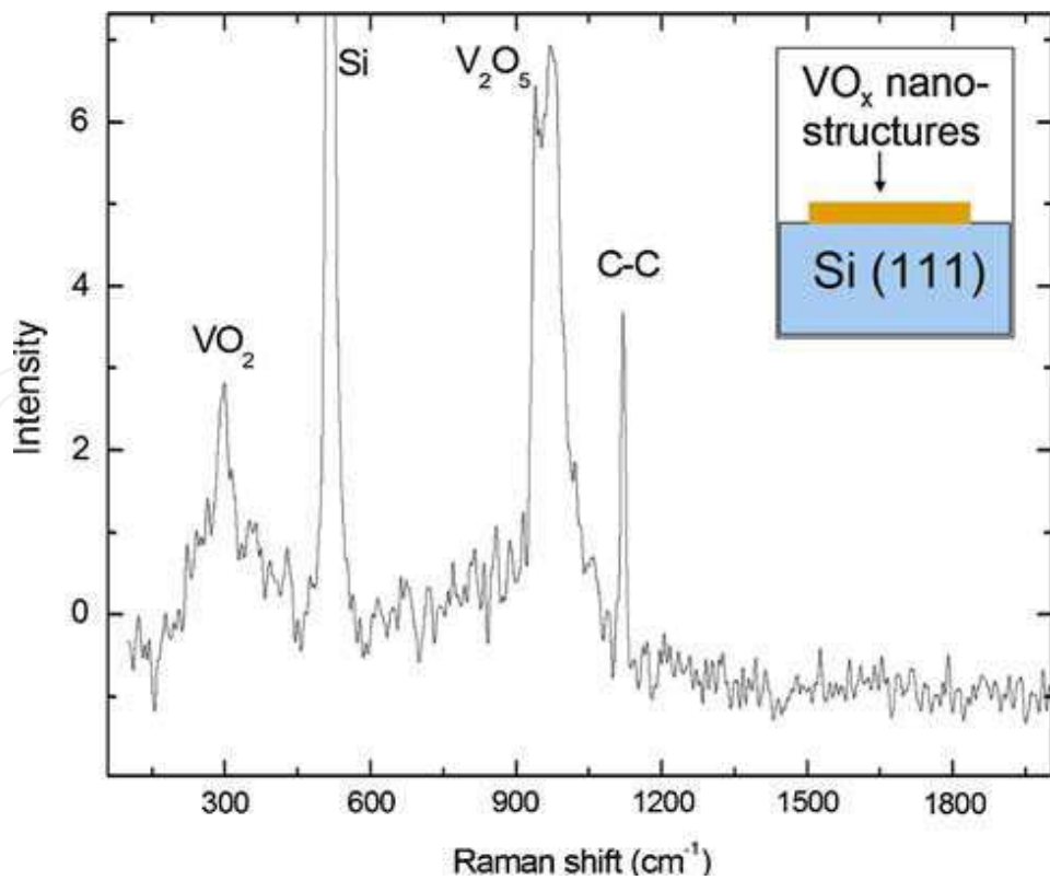
Fig. 15. Raman spectrum of inorganic fullerenes of \text{VO}_x nanostructures [52]
