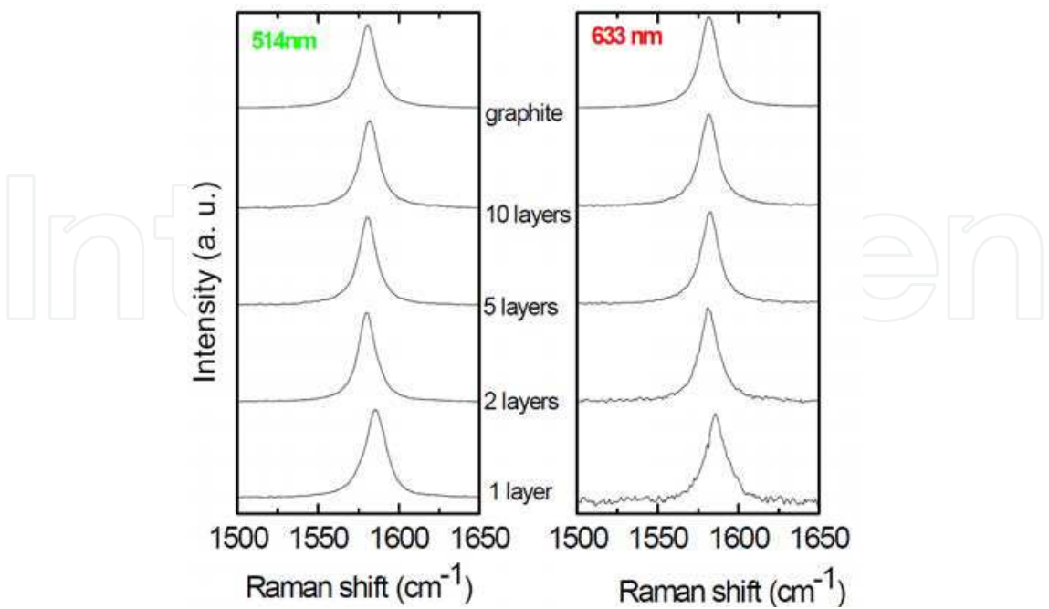
Fig. 8. The slight up-shift of the graphite G peak as the number of graphene layers decreases to one layer. (From A.C. Ferrari et al [7])
