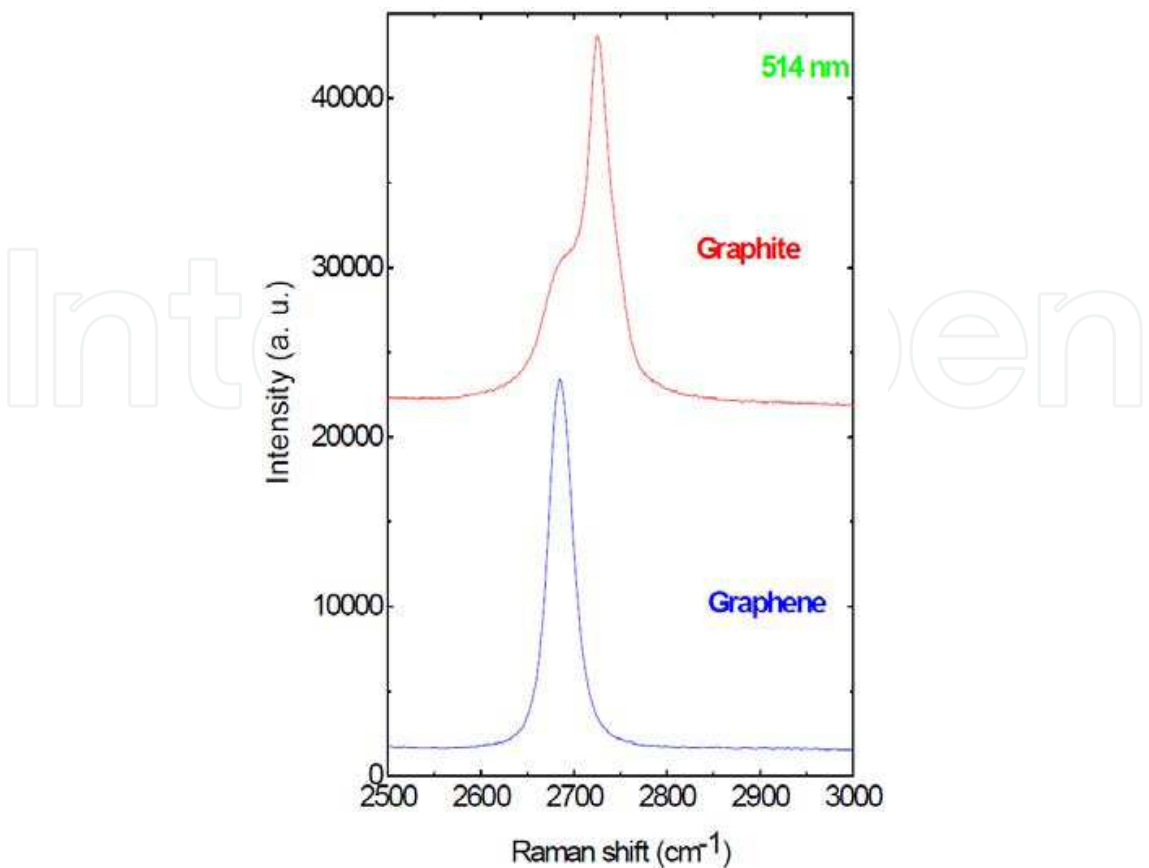
Fig. 7. The single 2690 cm -1 phonon from the one-layer graphene replaced by a main phonon at 2710 cm -1 with the 2690 cm -1 becoming its shoulder in multi-layer graphite (From A.C. Ferrari et al [7])
