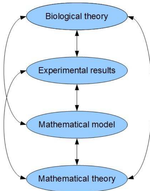
Fig. 1. Relationship among experiments, models, and theories.
