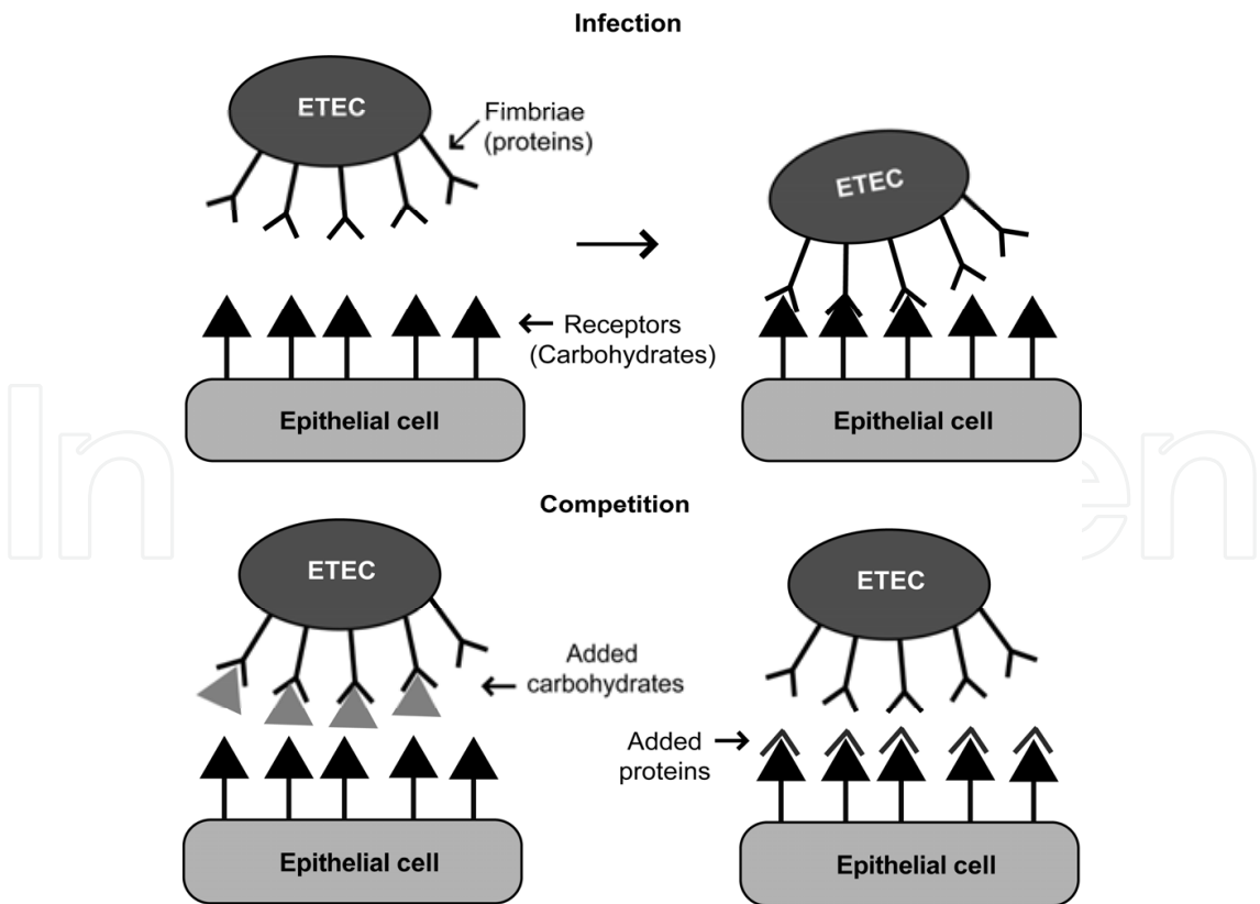
Fig. 5. Infection of intestinal tissue cells by ETEC bacteria and the mechanisms of inhibition of adhesion by specific food components.
