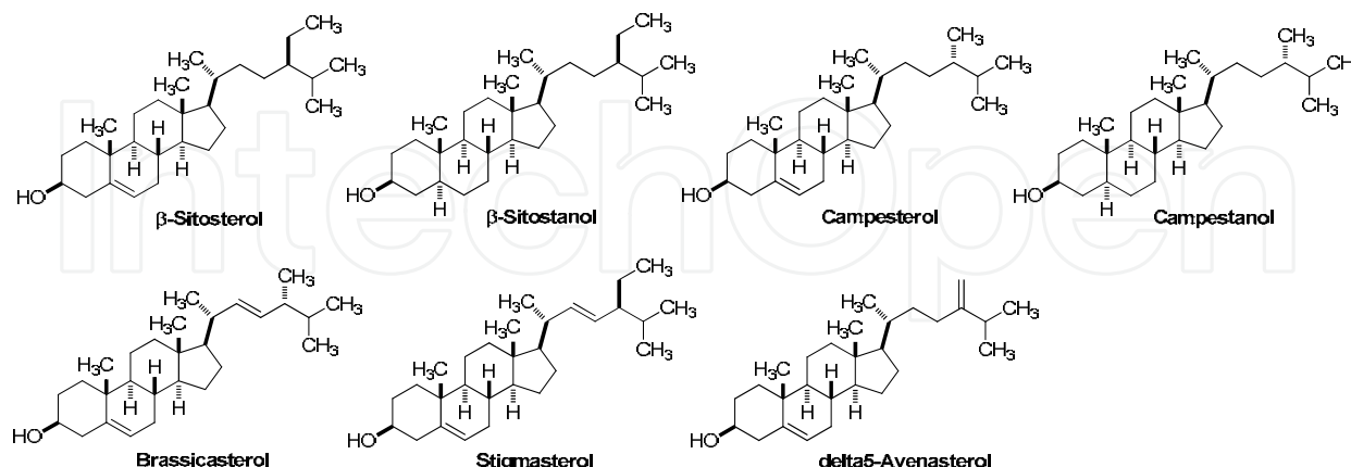
Fig. 6. Structures of plant sterols from soybeans
