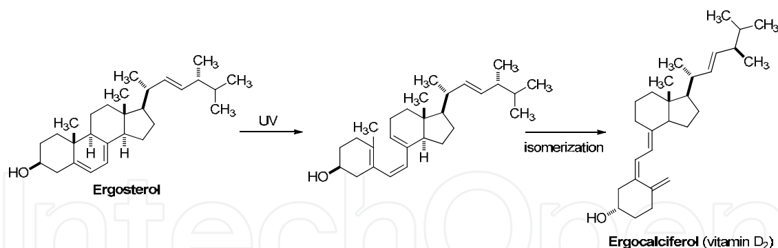
Scheme 2. Synthesis of ergocalciferol from ergosterol (vitamin D 2 )
