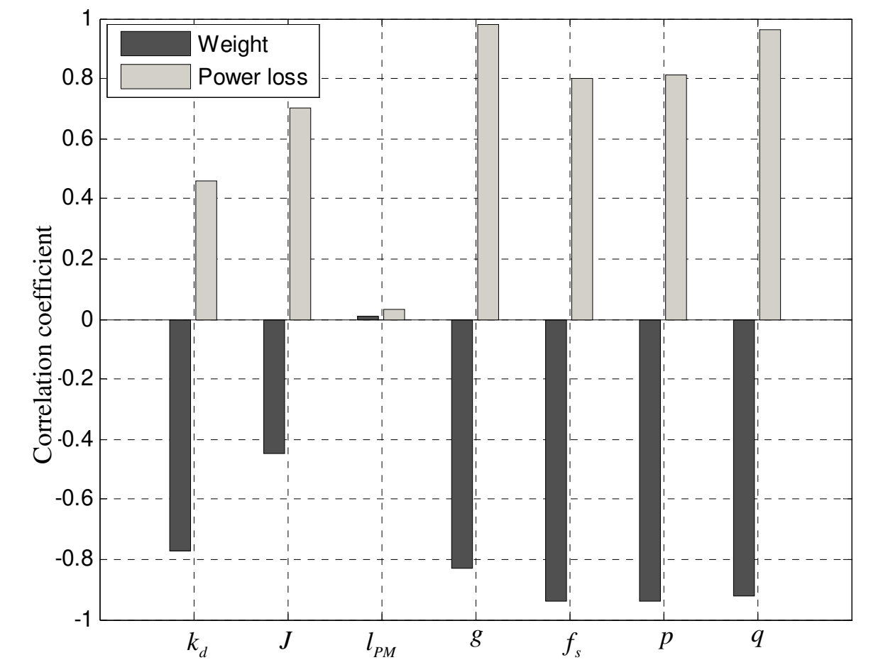
Fig. 16. Correlation between the optimization variables and the objective functions
