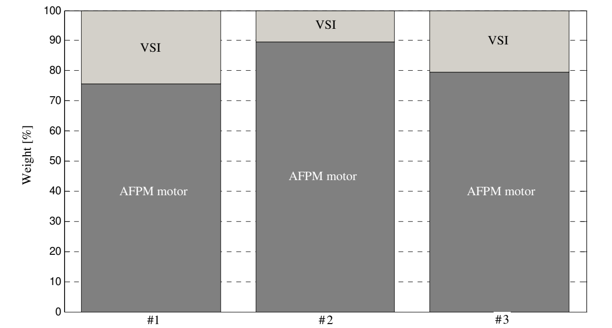
Fig. 17. Distribution of the weight among the AFPM motor and the VSI
