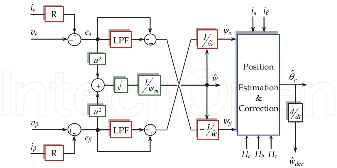
Fig. 7. Block diagram of the Back-EMF/Hall-effect based position and speed estimator.
