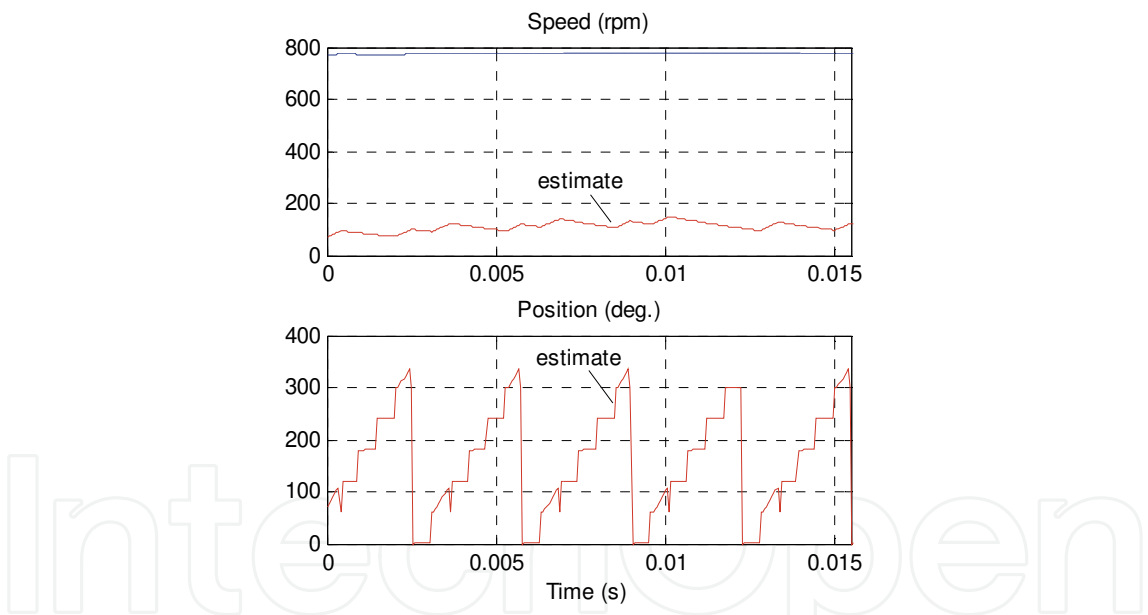
Fig. 6. Deterioration of the estimator at 780 rpm.
