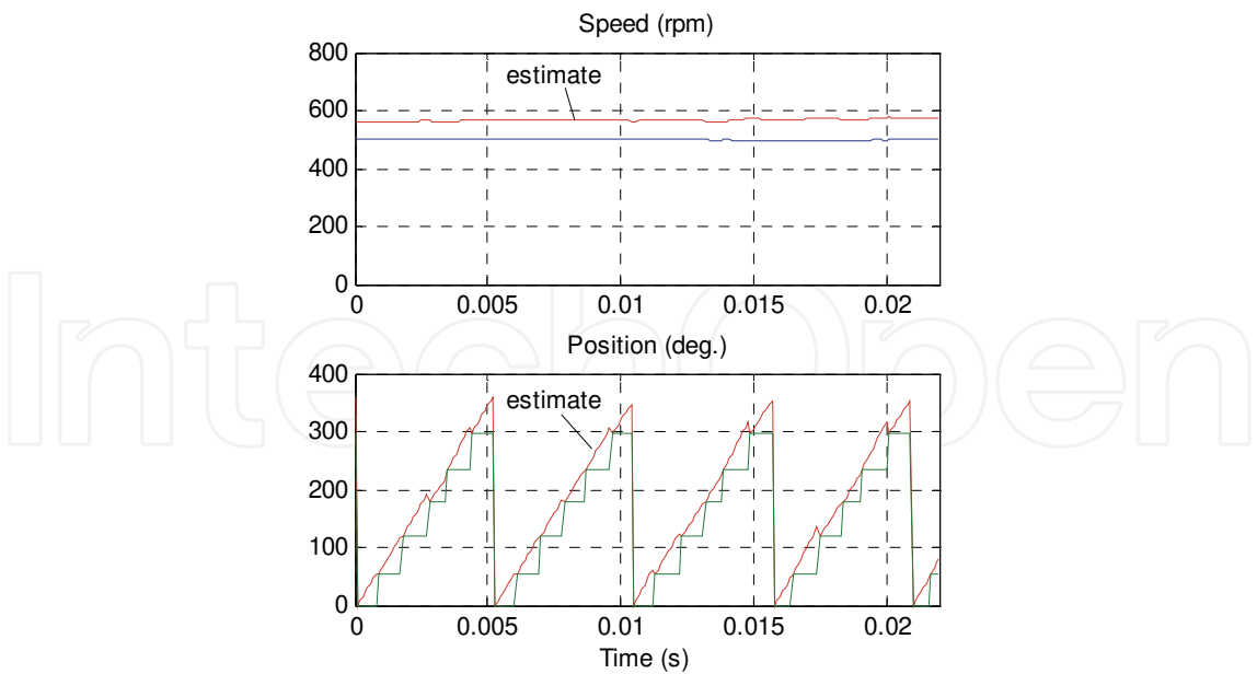
Fig. 5. Speed and 1 st order position estimates deviation during motor acceleration around 500 rpm.
