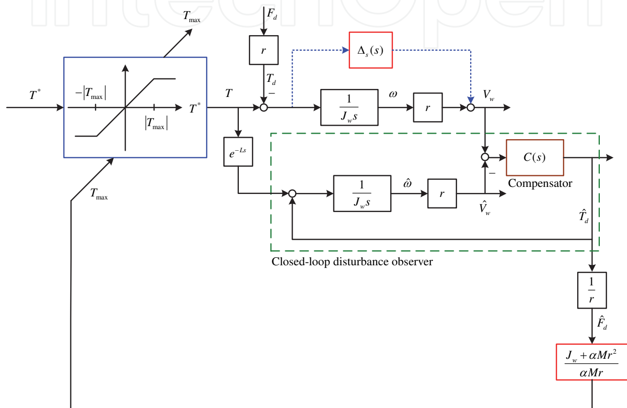
Fig. 8. Advanced MTTE control system.
