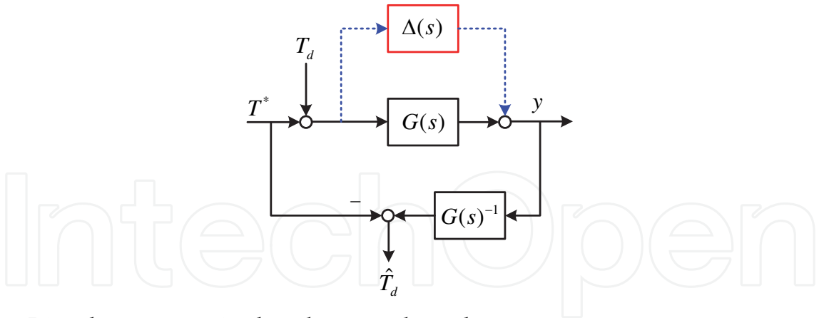
Fig. 4. Disturbance estimation based on open-loop observer.
