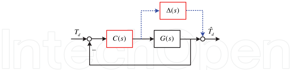
Fig. 6. Equivalent control block diagram of disturbance estimation.
