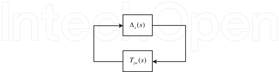
Fig. 10. Standard control configuration.
