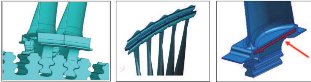
Fig. 1. Different types of friction contacts in turbine bladed disks: blade root joints, blade shrouds and underplatform dampers
