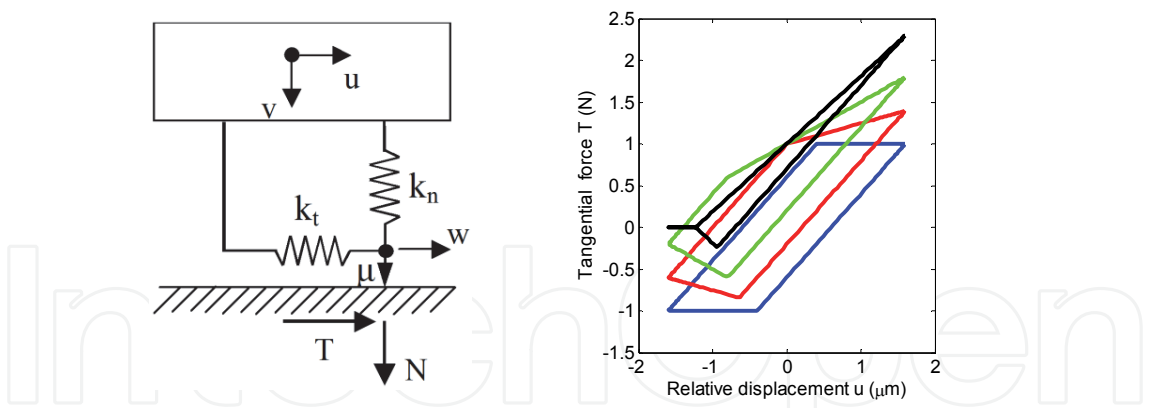
Fig. 7. 1D relative displacements and variable normal load: contact model (left) and typical hysteresis cycles (right)
