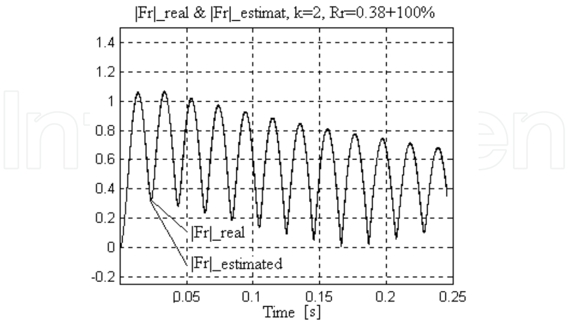
Fig. 6. Comparative presentation of the estimated (forward of the output filter) and the real rotor flux modulus.
