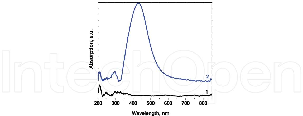
Fig. 6. UV-visible absorption spectra of the synthesized DNDs: (1) 6-DND; (2) Ag-DND;
