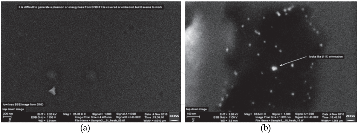
Fig. 9. Low loss BSE imaging from DND particles, embeded inside the Si-DND/PPHMDS layer (a); Low loss BSE imaging of the Si-DND/PPHMDS surface (b).
