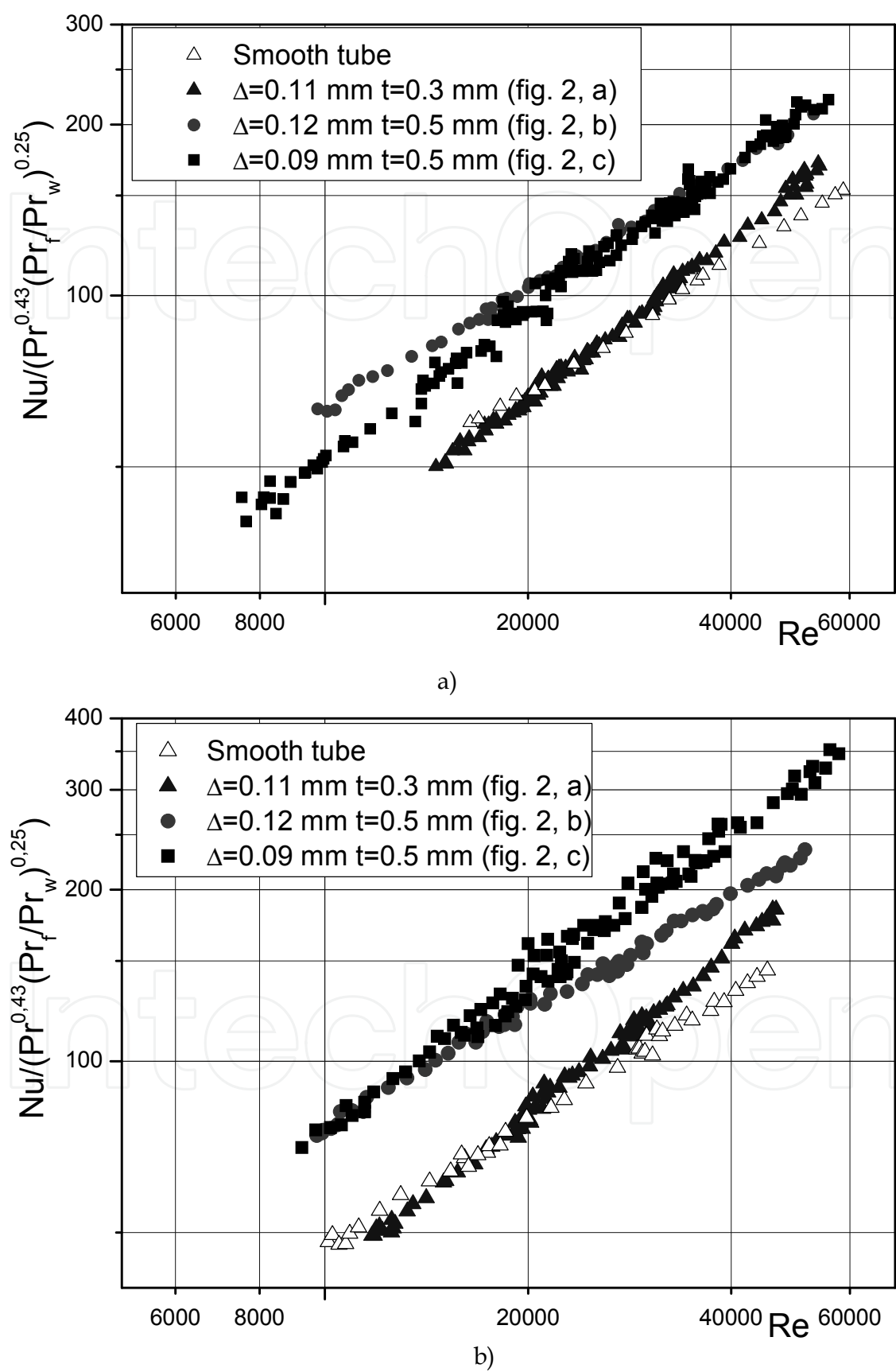
Fig. 11. Heat transfer of rough tubes with twisted tape insert: a) S/d=6 , b) S/d=2.5
