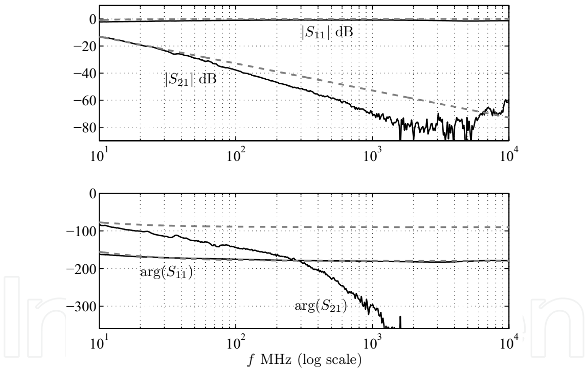
Fig. 9. Selection of the scattering responses of the VDD-VSS structure. Solid lines: reference measured responses; dashed lines: responses of lumped capacitor Z_e(s) = 1/sC .
