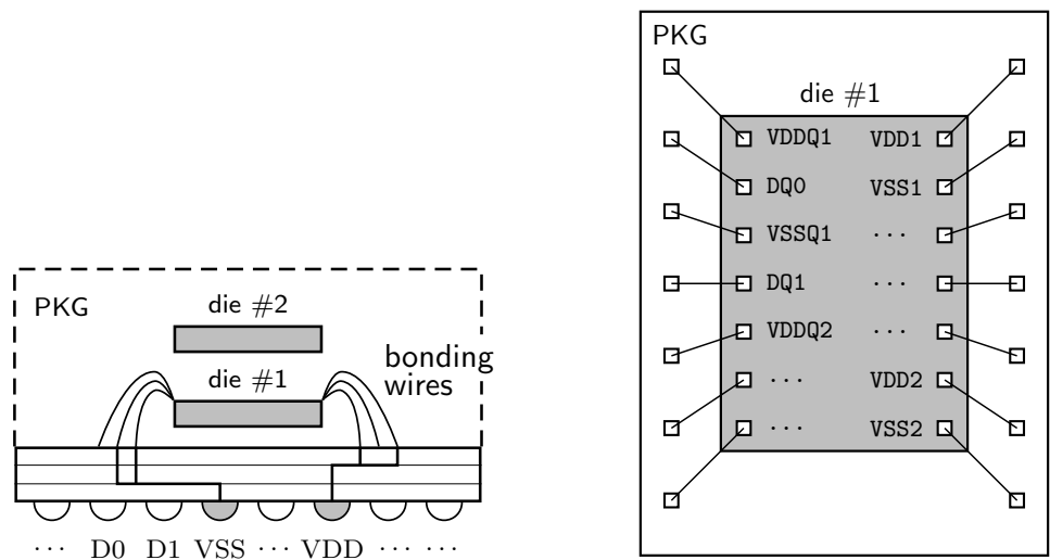
Fig. 1. Typical structure of a memory chip (i.e., the die #1) encapsulated in package. Left panel: side view; right panel; top view.
