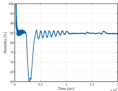
Fig. 7. Relative humidity with a packaged PID: 85 % RH
