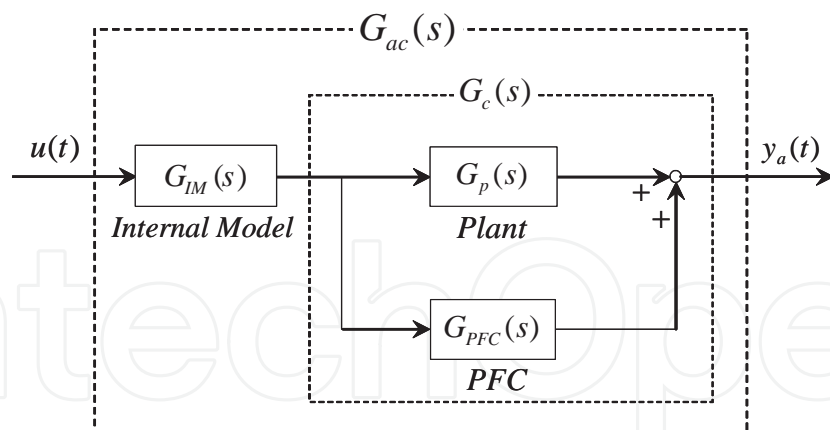
Fig. 3. Block diagram of a modified augmented system
