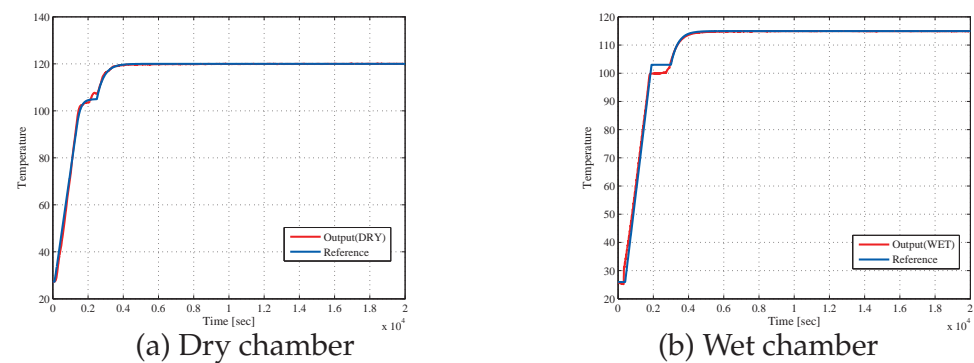
Fig. 11. Comparison between Output and Reference signal: 120 degree and 85 % RH
