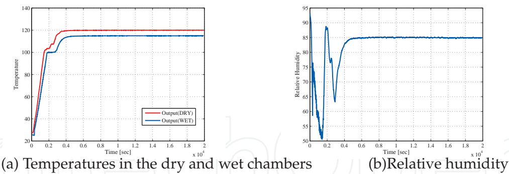
Fig. 10. Experimental results of outputs: 120 degree and 85 % RH
