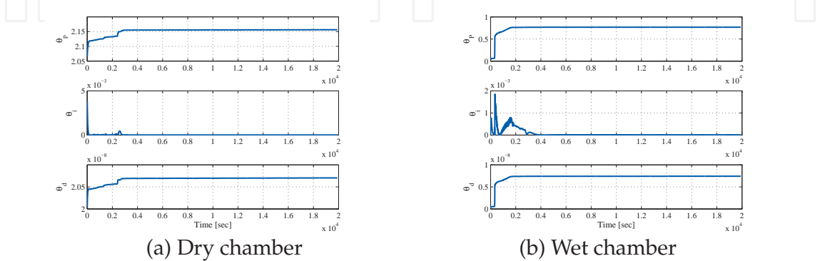
Fig. 17. Adaptively adjusted PID gains: 130 degree and 85 % RH
