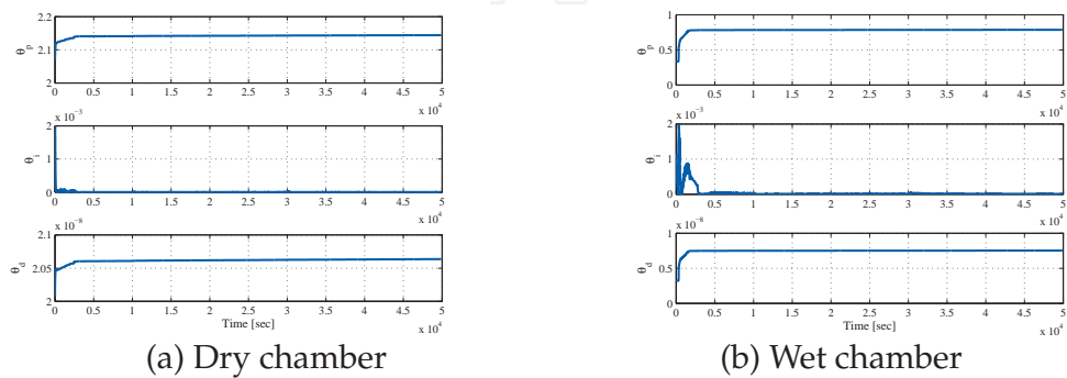
Fig. 25. Adaptively adjusted PID gains: 120 \rightarrow 130 \rightarrow 120 degree with 85 % RH
