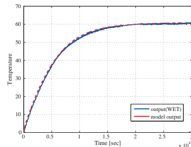
(b) Temperature in the wet chamber
