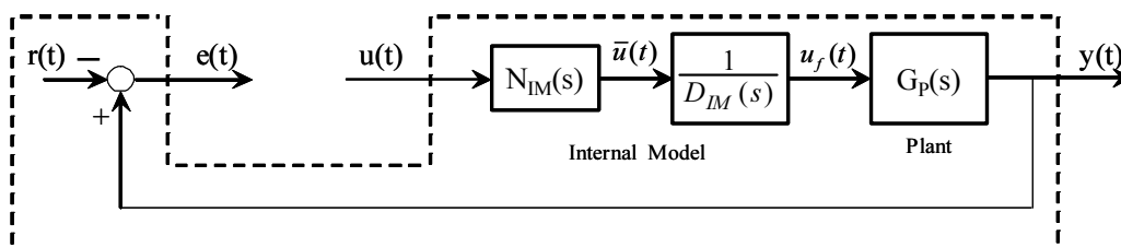
Fig. 1. Error System
