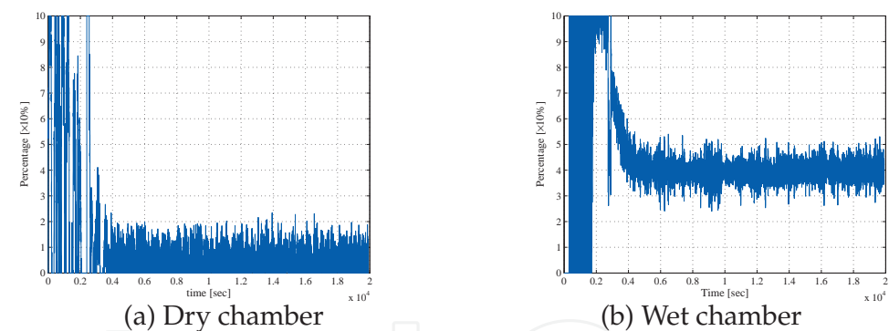
Fig. 12. Control Input: 120 degree and 85 % RH
