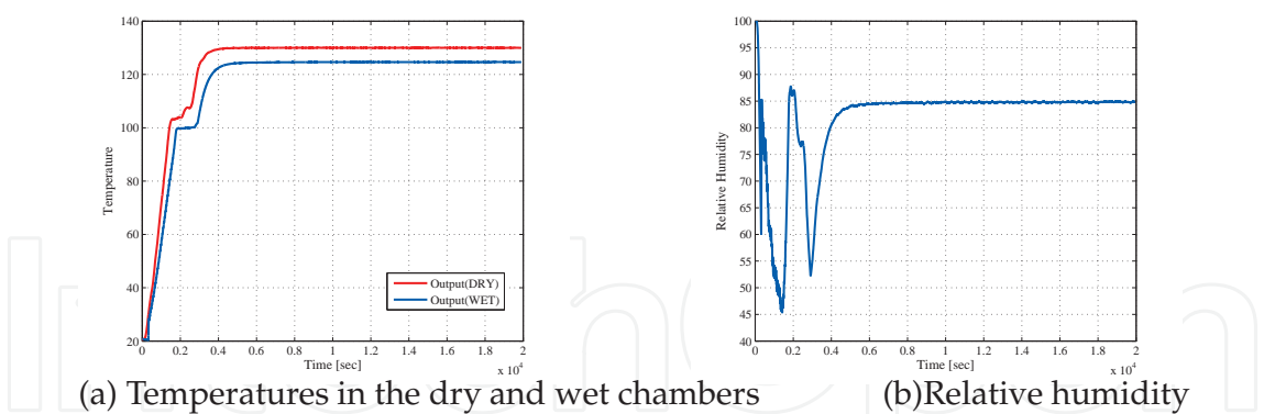
Fig. 14. Experimental results of outputs: 130 degree and 85 % RH
