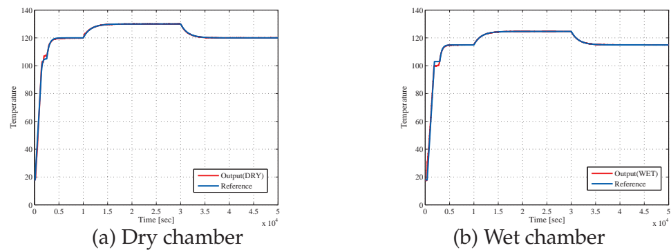
Fig. 23. Comparison between Output and Reference signal: 120 \rightarrow 130 \rightarrow 120 degree with 85 % RH
