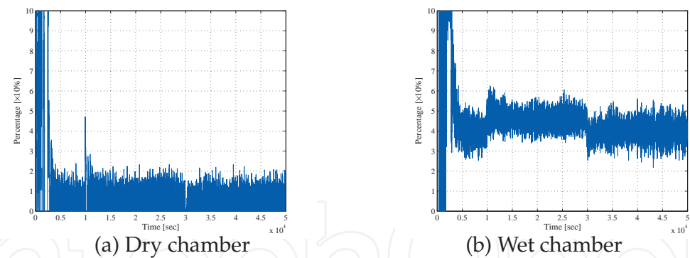
Fig. 24. Control Input: 120 \rightarrow 130 \rightarrow 120 degree with 85 % RH
