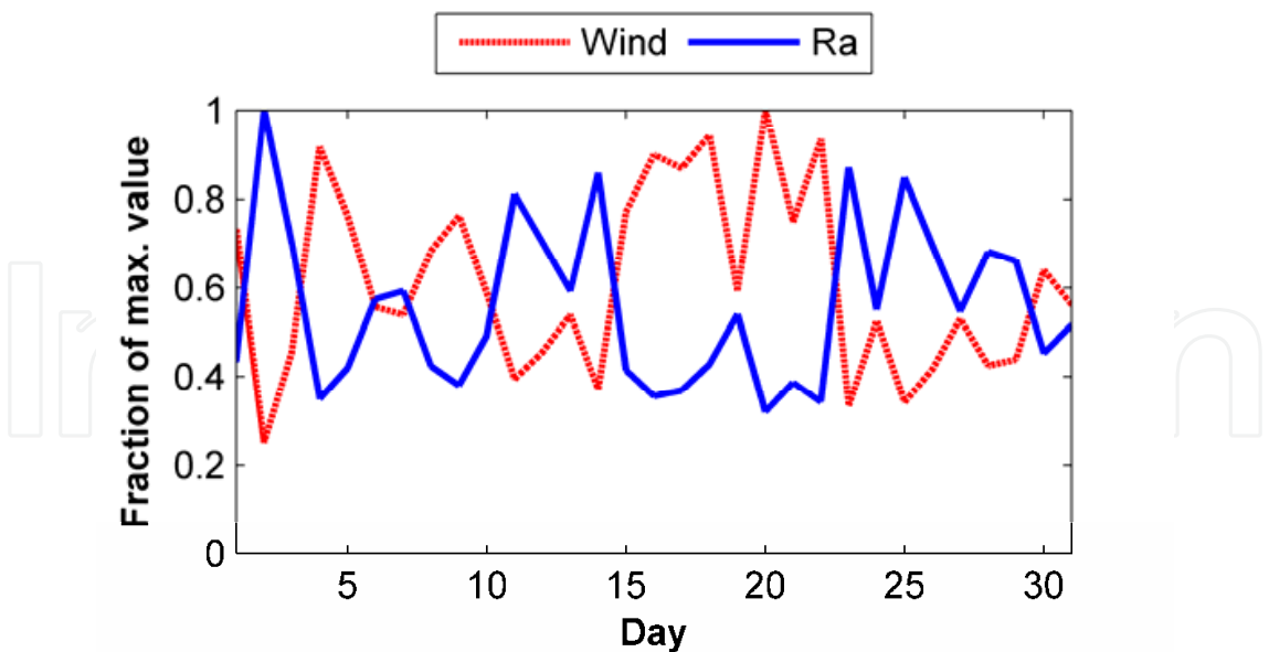
Fig. 6. Variation of aerodynamic resistance with wind speed (Dec 2008 14:30 IST)
