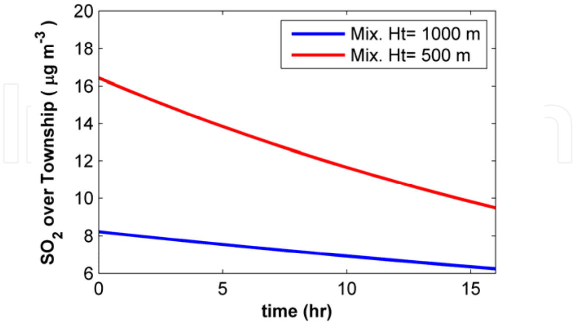
Fig. 11. Depletion of residual SO 2 concentration over the township considering the higher deposition velocity of October
