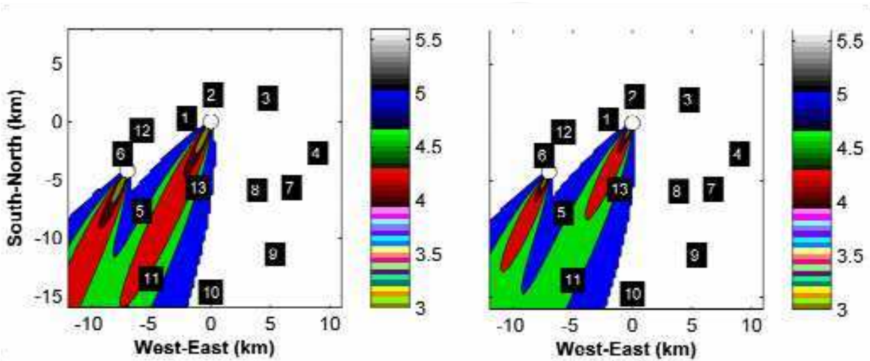
Fig. 18. Contours of the rain water pH for rain rates of 10 mm hr -1 (left) and 100 mm hr -1
