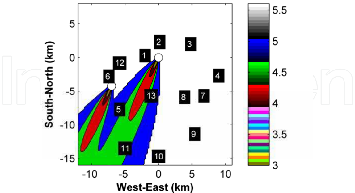
Fig. 17. Contours of the rain water pH at the ground for a rain rate of 43.2 mm hr -1
