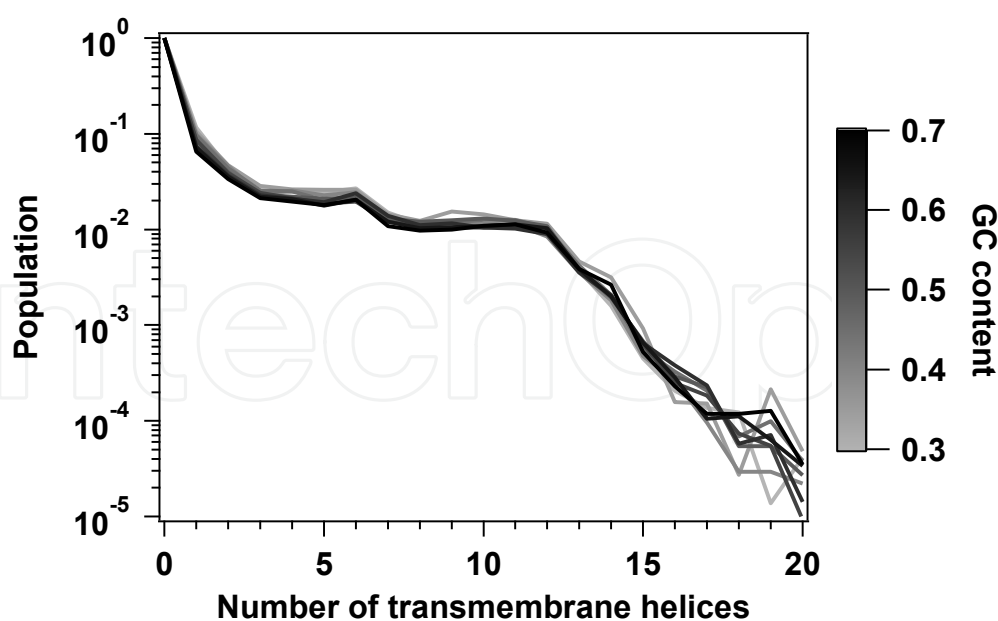
Fig. 3. Number distributions in nine groups of organisms classified by GC content. 557 prokaryotes were divided into nine groups according to GC content (0.3, 0.35, 0.4, 0.45, 0.5, 0.55, 0.6, 0.65 and 0.7).
