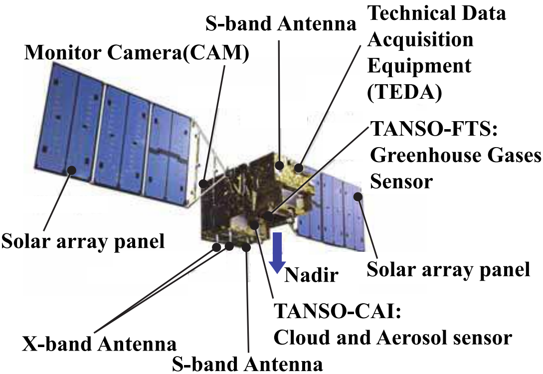
Fig. 3. Overall view of GOSAT
