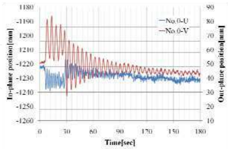
Fig. 17. Measurement result of marker No. 0
