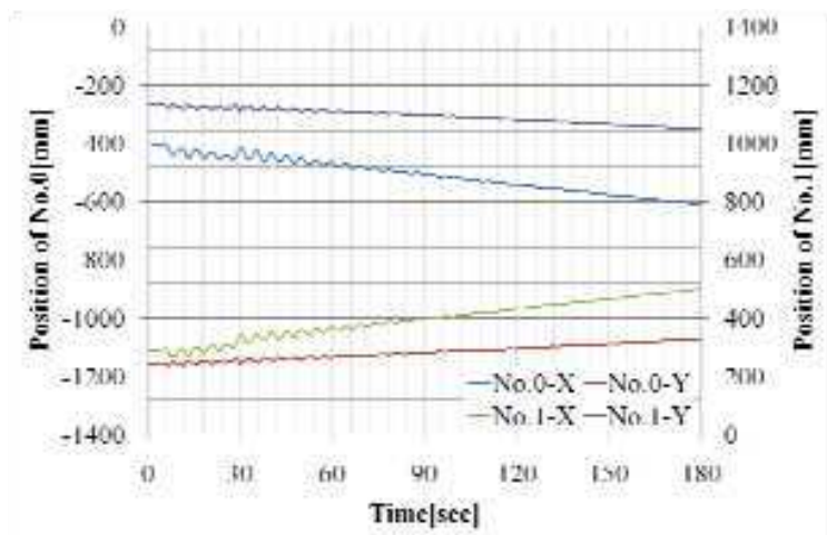
Fig. 16. The transition of the marker position as shown by the world coordinate frame
