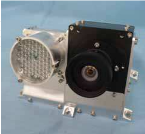
Fig. 4. Monitoring camera mounted on GOSAT © Meisei Electric Co., Ltd.
