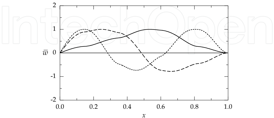
Fig. 8. First three mode shapes obtained from Eq. (3.25). The solid, dashed, and dotted curves represent the 1 st , 2 nd , and 3 rd modes, respectively.
