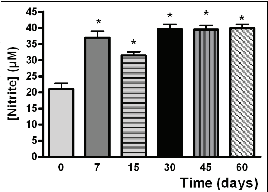
Fig. 7. Nitrite concentration in the optic nerve head at different times. Data are mean ± SEM. * p <0.001. Experimental glaucoma model was performed at time 0
