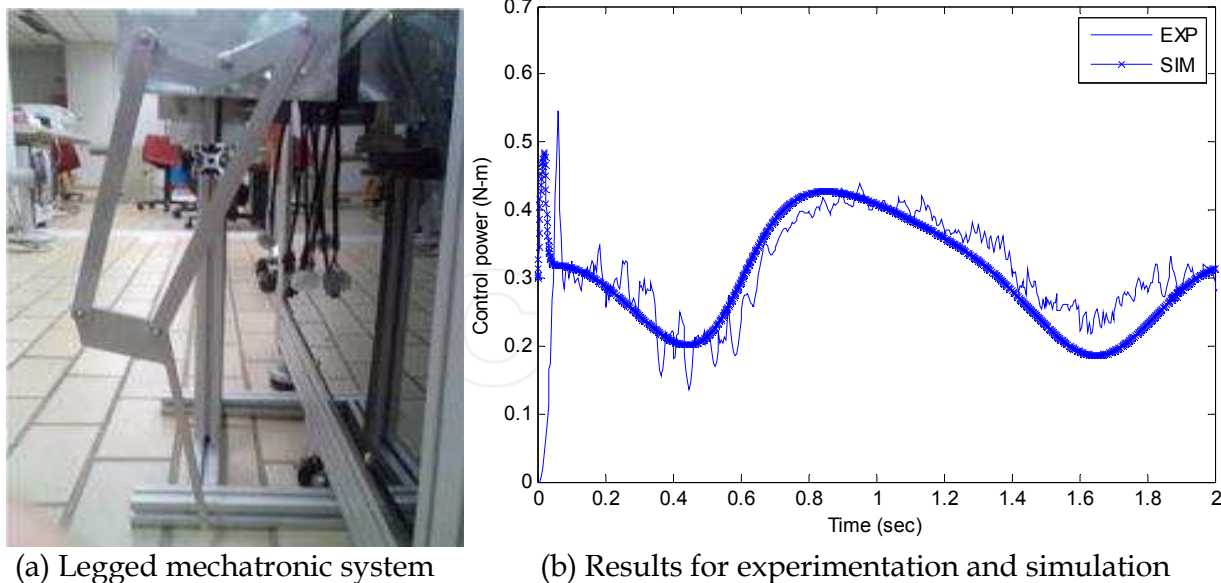
Fig. 12. Legged mechatronic.
