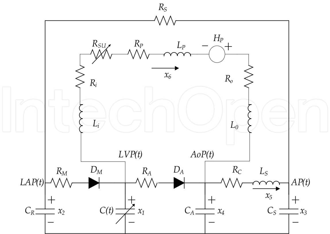
Fig. 3. Combined cardiovascular and LVAD model
