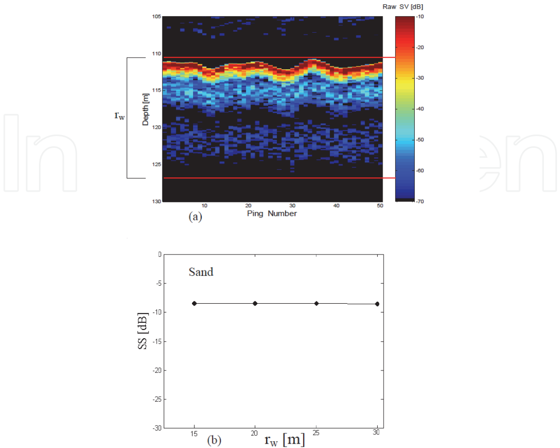
Fig. 4.3. The echogram in raw SV scale (a) and the relation of measured SS on r_w values (b).
