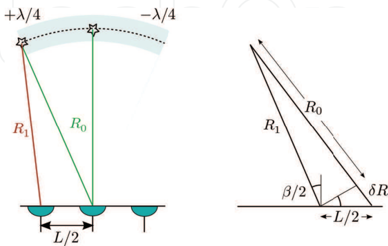
Fig. 4. Geometrical derivation of angular resolution.
