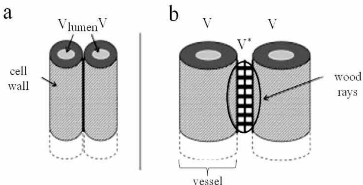
Fig. 8. Representation of two adjacent wood vessels in untreated wood (a) compared to WPC (b) and localization of the fracture propagation V and V^*
