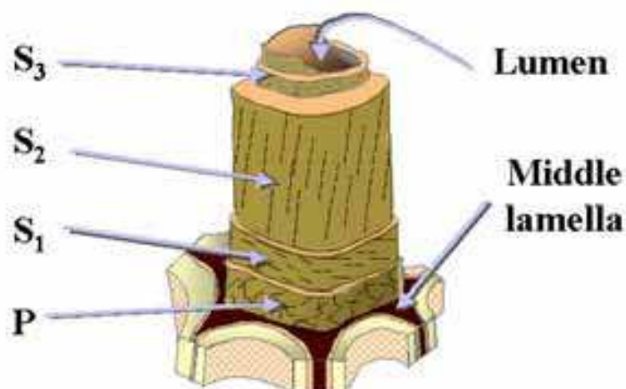
Fig. 3. Ultrastructure of the wood cell wall
