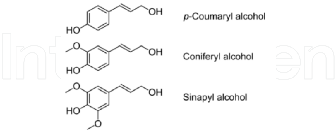
Fig. 5. Monolignol structures
