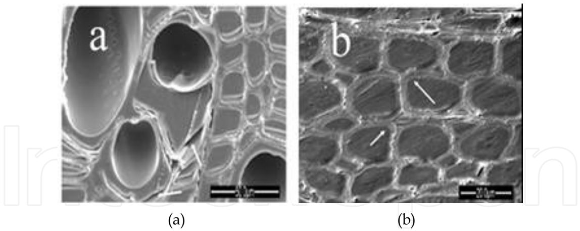
Fig. 12. SEM morphologies of WPCs prepared from MMA monomer(s) (a) WPC made with MMA monomer (b) WPC made with MMA with GMA or/and anhydride as cross-linker
