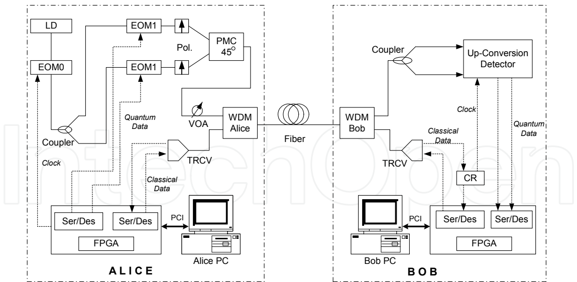
Fig. 4. The B92 polarization coding QKD system. LD: Laser diode; EOM: Electric-optic modulator (LiNbO3); PC: Polarization controller; PMC-45°: Polarization maintaining combiner that combines two light signals that are separated by 45 degrees; VOA: Variable optical attenuator; WDM: Wavelength-division multiplexer; SMF: Standard single-mode fiber; TRCV: Optical transceiver; CR: Clock recovery module; FPGA: Custom printed circuit board controlled by a field-programmable gate array; PCI: PCI connection; Dotted line: Electric cable; Solid line: Optical fiber.
