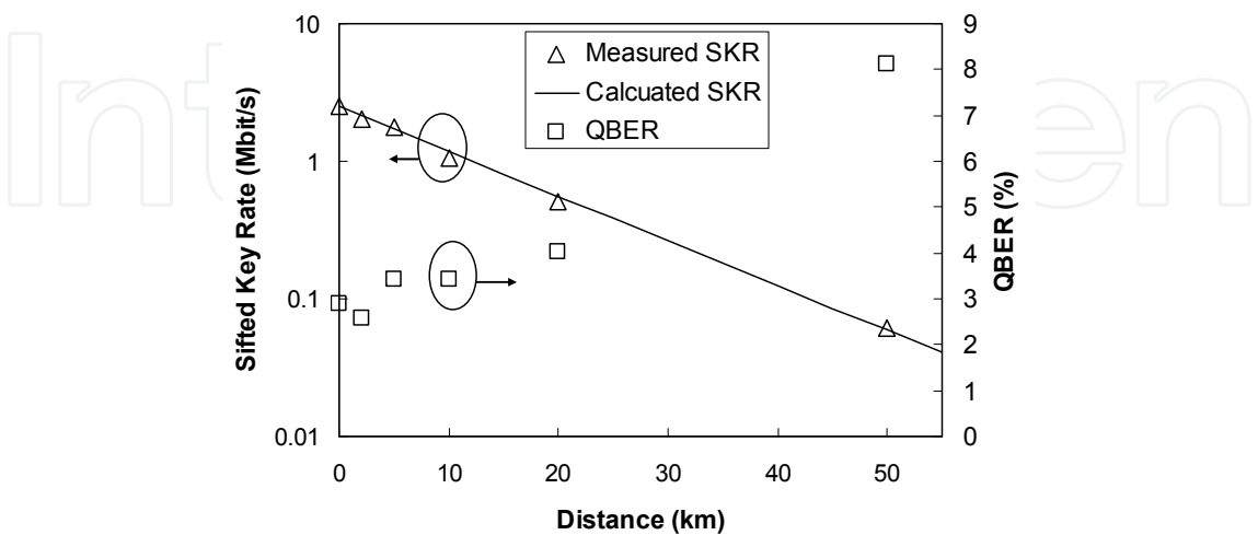
Fig. 5. The system performance of the B92 polarization-based QKD system using pulsed pump up-conversion detectors.
