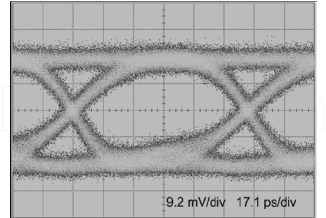
Fig. 20. Eye diagram of back-to-back test for an SMA-packaged device operated at -5 V and 10.3 Gb/s with PRBS of 2^{31}-1 word length at 1.3\text{ }\mu\text{m} wavelength.
