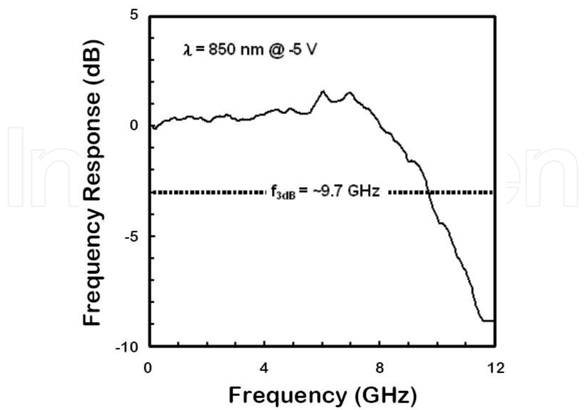
Fig. 13. Device characteristics in frequency response at the 850 nm wavelength.
