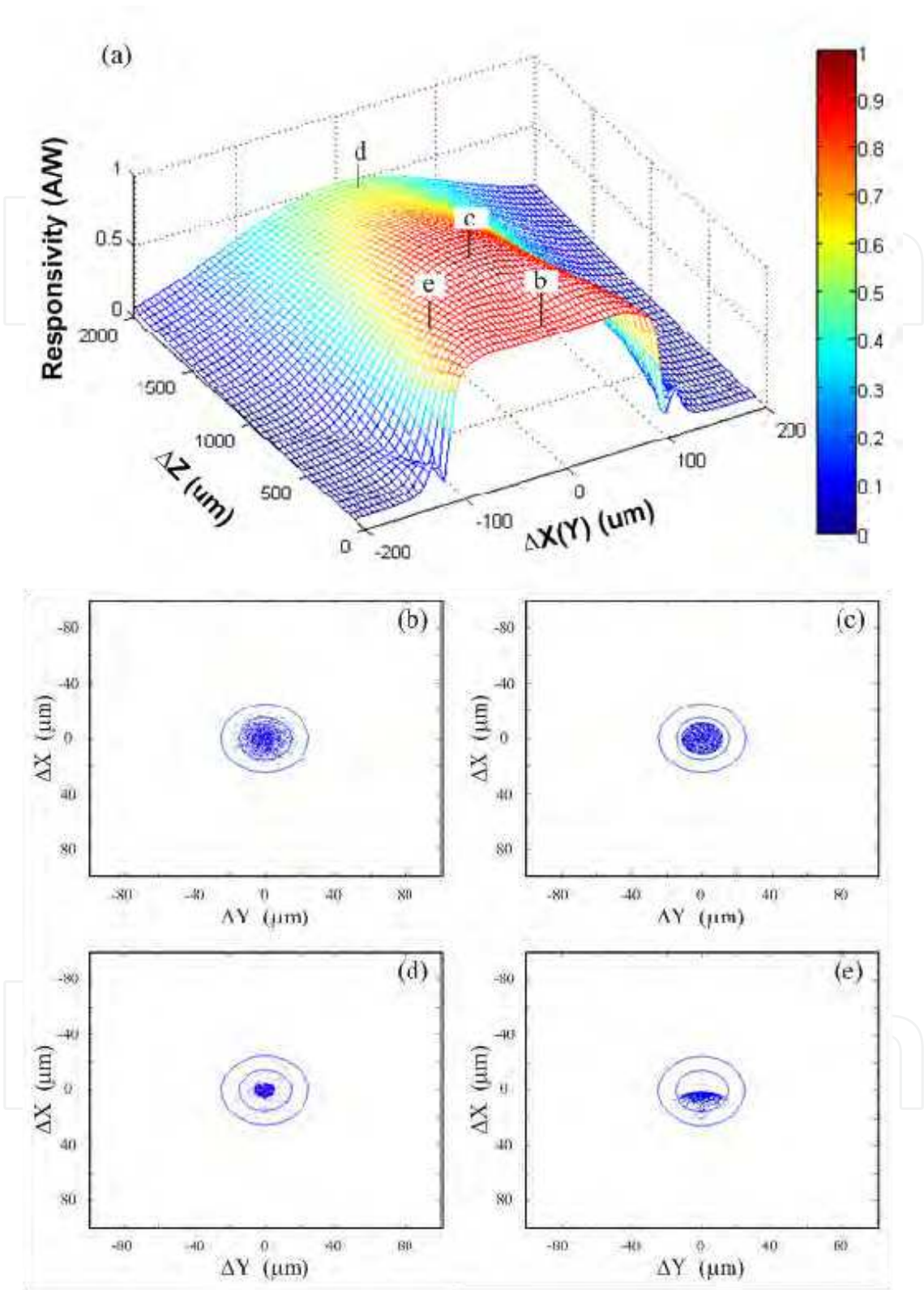
Fig. 18. (a) Modeling two-dimensional response uniformity of the \phi = 250\text{-}\mu\text{m} ruby MBL-integrated PD ( H = 50\text{ }\mu\text{m} ) across the X-Z plane. The ray trace maps are derived from the positions ( \Delta X and \Delta Z in \mu\text{m} ), (b) (0, 200), (c) (0, 800), (d) (0, 1900), and (e) (-80, 300) labeled on the responsivity surface.
