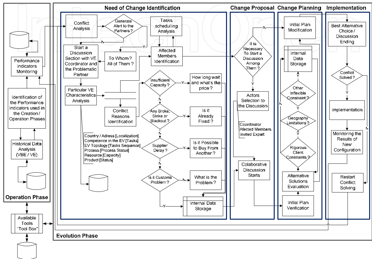
Fig. 4. Basis Protocol for the VE Evolution Management.
