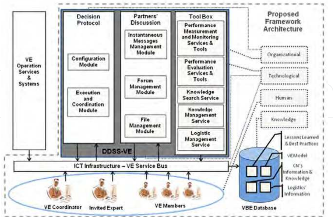
Fig. 3. Framework Architecture.
