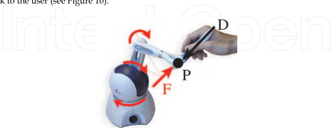
Fig. 10. Commercially available haptic device. The haptic device is driven by the position ( \mathbf{P} ) and direction ( \mathbf{D} ) of the stylus that are determined by the user's movements, and renders back a force ( \mathbf{F} ) processed by the computer.
