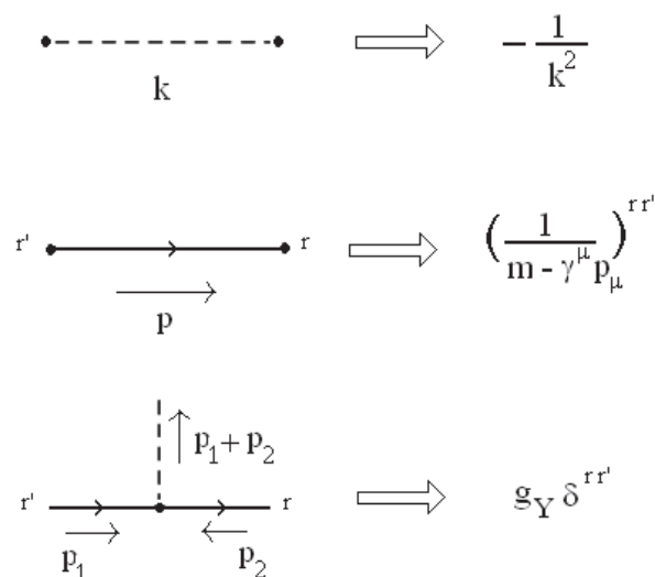
Fig. 5. The figure illustrates the Feynman rules for the particular Yukawa model approximation adopted for the Dilaton action in Ref. (33)
