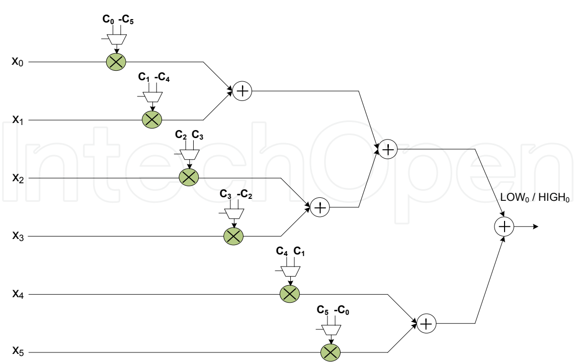
Fig. 1. FP-based DAUB6 filter architecture.
