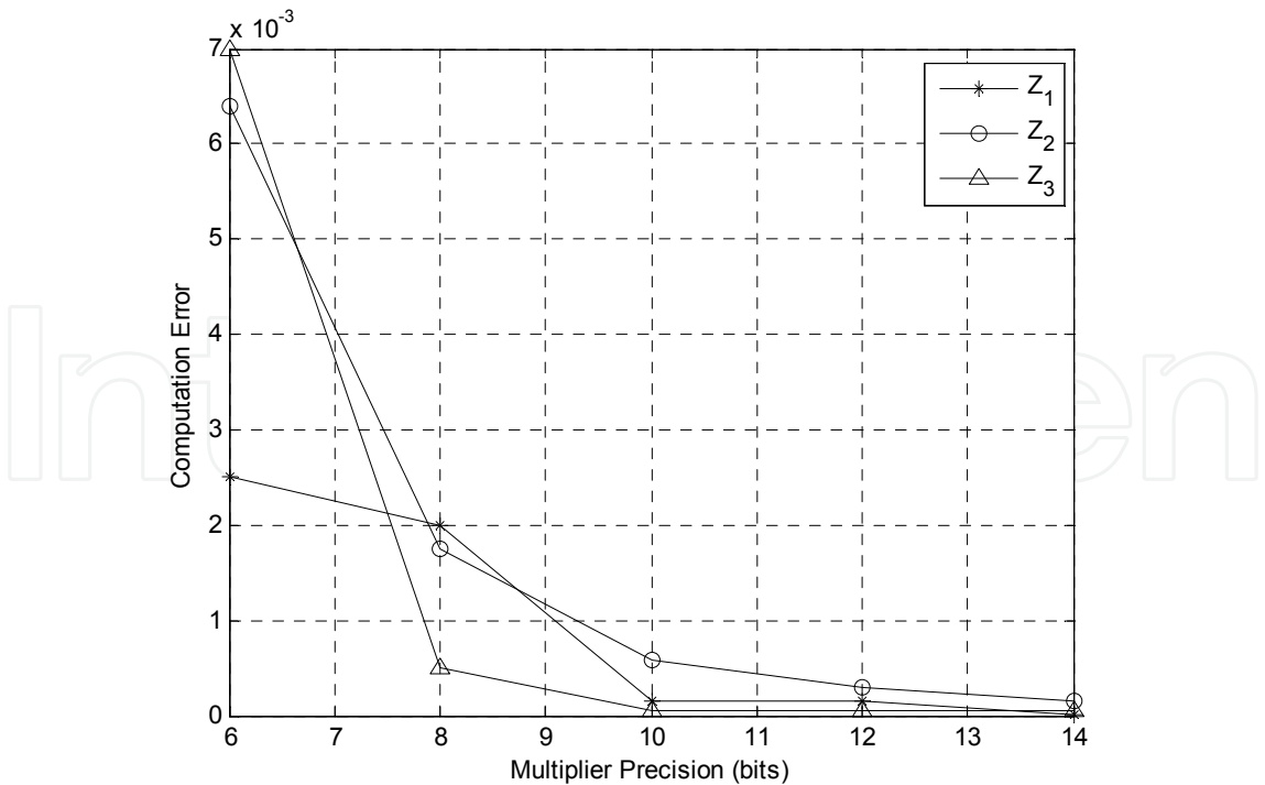
Fig. 4. Computation error in AIQ multipliers.
